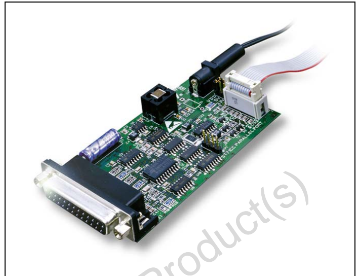
Figure 1: ST7-STICK Programmer
