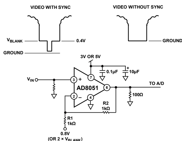
Figure 51. Sync Stripper
