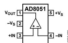
Figure 2. SOT-23-5 (RJ)
