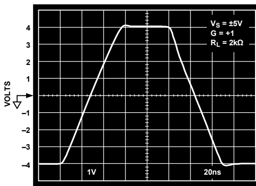
Figure 39. Large Signal Step Response; V_S = \pm 5 \text{ V} , G = +1
