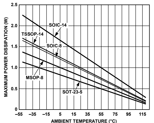
Figure 6. Maximum Power Dissipation vs. Temperature for AD8051/AD8052/AD8054
