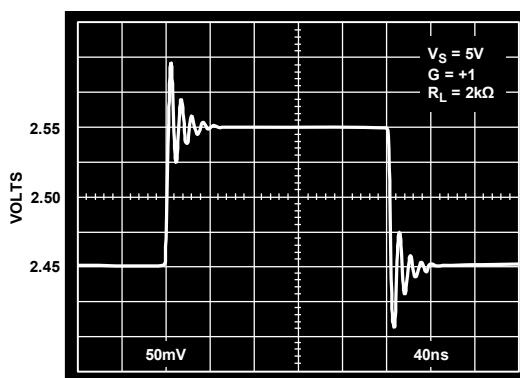
Figure 38. AD8054 100 mV Step Response; V_S = 5 \text{ V} , G = +1
