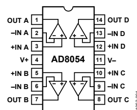
Figure 4. SOIC (R-14) and TSSOP (RU-14)
