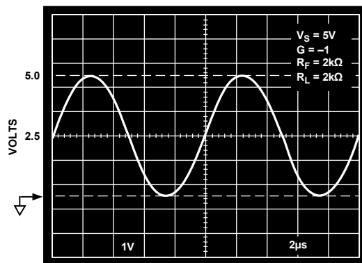
Figure 37. Output Swing; G = -1 , R_L = 2 \text{ k}\Omega
