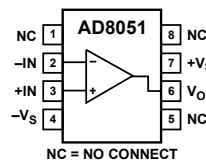
Figure 1. SOIC-8 (R)
