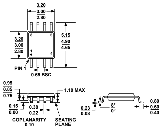
Figure 55. 8-Lead Mini Small Outline Package [MSOP] (RM-8)
