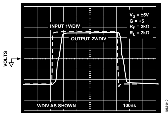
Figure 41. Overdrive Recovery
