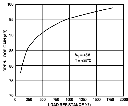
Figure 7. Open-Loop Gain vs. R_L to +2.5 V
