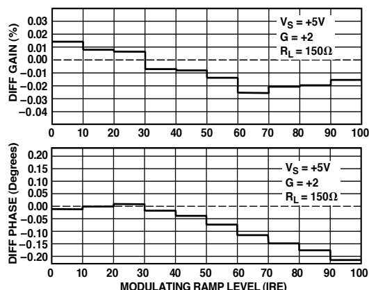
Figure 13. Differential Gain and Phase Errors
