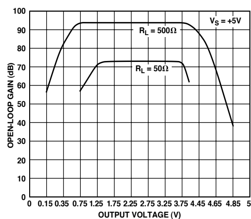
Figure 9. Open-Loop Gain vs. Output Voltage
