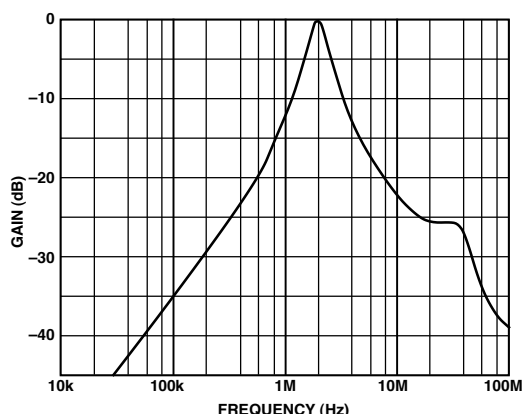
Figure 39. Frequency Response of 2 MHz Band-pass Biquad Filter
