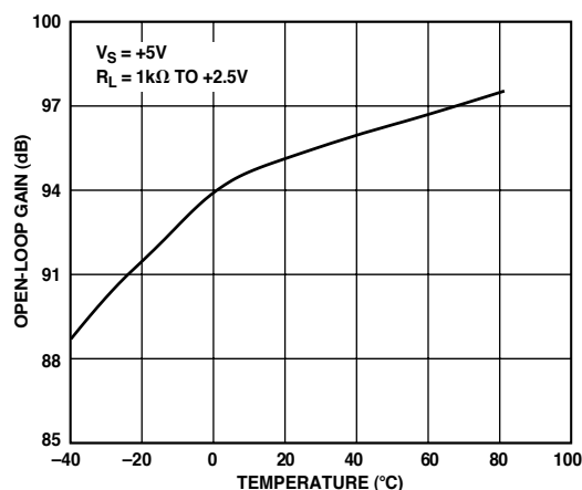
Figure 8. Open-Loop Gain vs. Temperature
