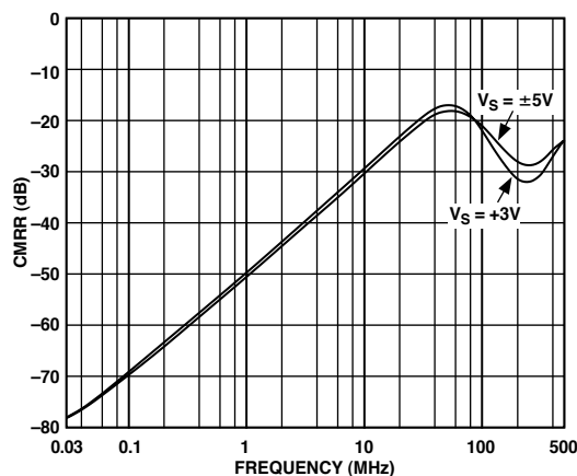
Figure 20. CMRR vs. Frequency
