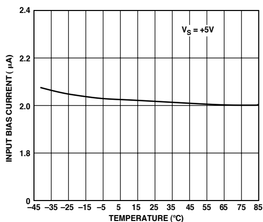
Figure 6. I_B vs. Temperature
