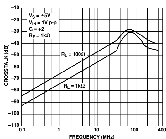
Figure 27. Crosstalk (Output to Output) vs. Frequency
