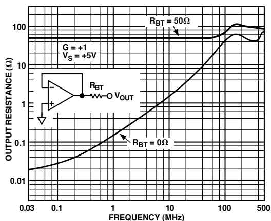
Figure 18. Output Resistance vs. Frequency
