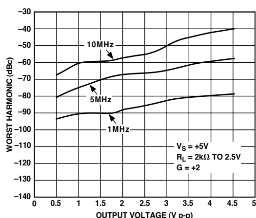
Figure 12. Worst Harmonic vs. Output Voltage
