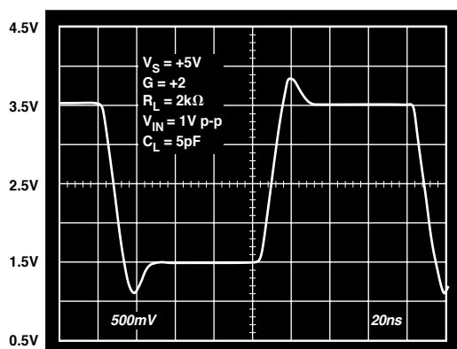
Figure 29. One Volt Step Response, V_S = +5\text{V} , G = +2
