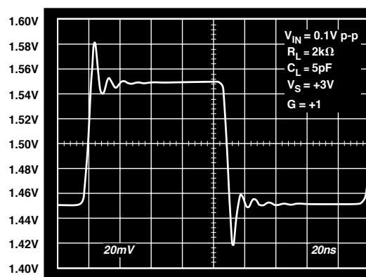
Figure 32. Step Response, G = +1 , V_{IN} = 100\text{mV}
