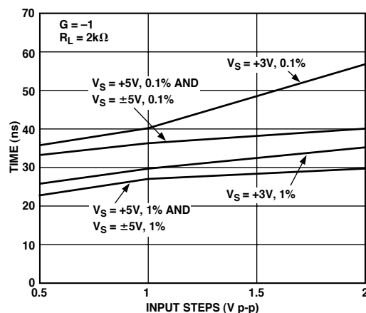
Figure 19. Settling Time vs. Input Step
