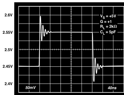
Figure 30. 100 mV Step Response, V_S = +5\text{V} , G = +1
