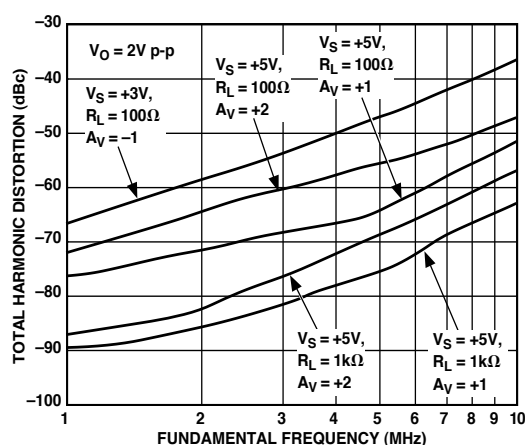
Figure 11. Total Harmonic Distortion
