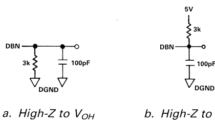
Figure 3. Load Circuits for Access Time Test ( t_{13} )
