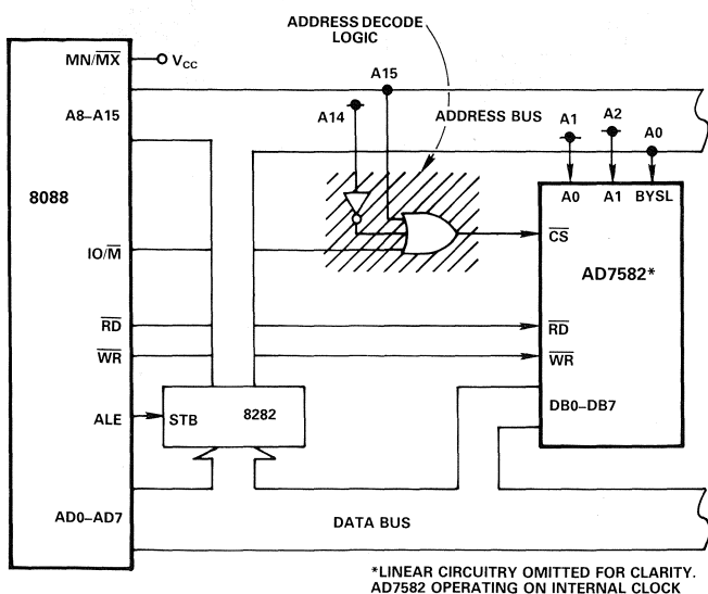
Figure 21. AD7582 – 8088 Interface
