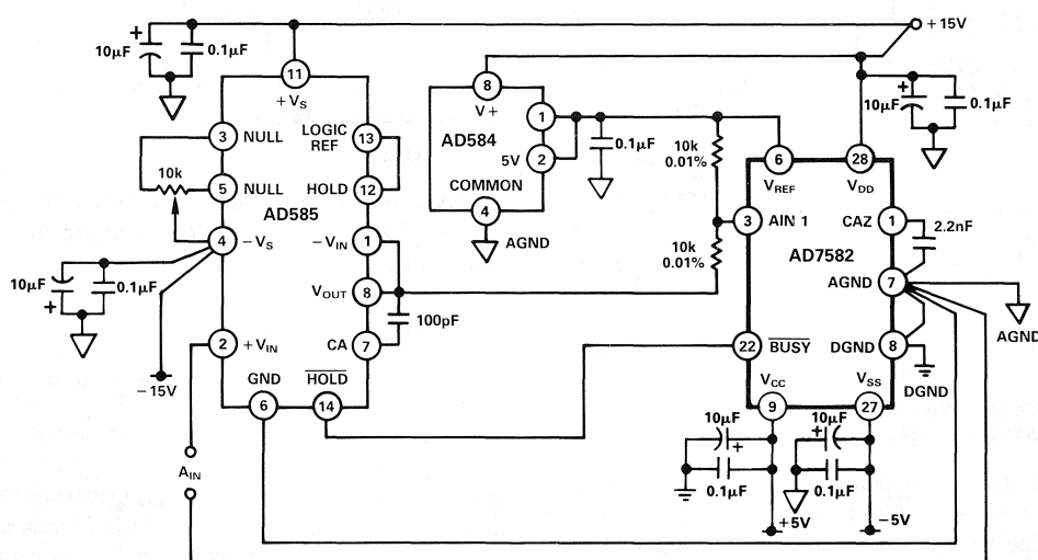
Figure 23. AD7582-AD585 Interface
