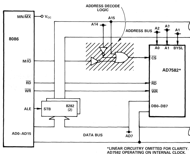
Figure 22. AD7582 – 8086 Interface
