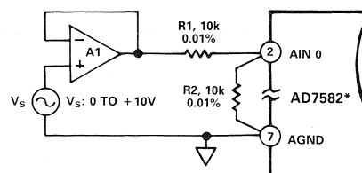
Figure 13. Unipolar 0 to +10V Operation
