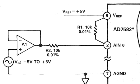
Figure 14. Bipolar -5V to +5V Operation
