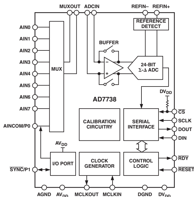
Figure 4. Block Diagram
