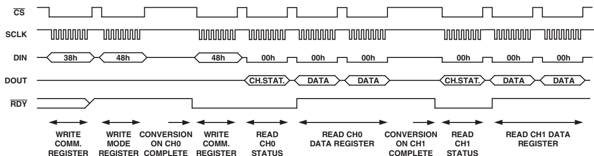
Figure 12. Continuous Conversion CH0 and CH1, Continuous Read
