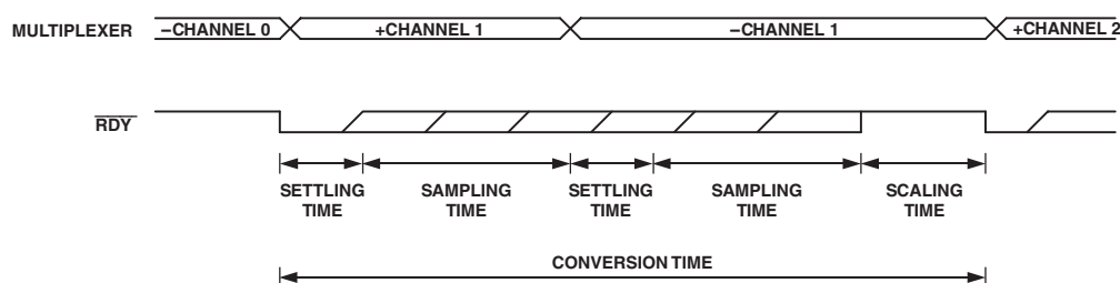
Figure 14. Multiplexer and Conversion Timing—Continuous Conversion on Several Channels with Chopping Enabled
