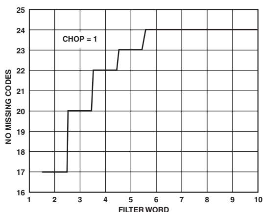
TPC 1. No Missing Codes Performance, Chopping Enabled
