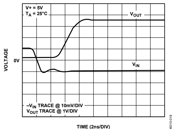
Figure 21. Rising Edge Response
