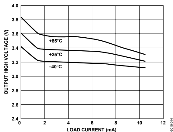
Figure 17. Output High Voltage vs. Load Current (Sourcing) Over Temperature
