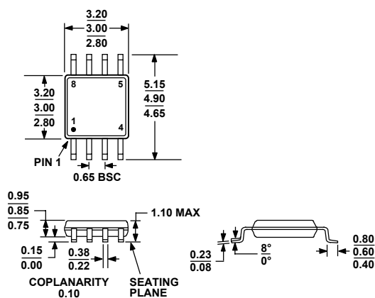
Figure 27. 8-Lead Mini Small Outline Package [MSOP] (RM-8)
