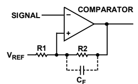
Figure 24. Configuring the AD8611/AD8612 with Hysteresis
