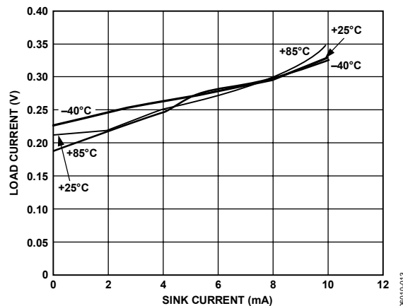
Figure 16. Output Low Voltage vs. Load Current (Sinking) Over Temperature
