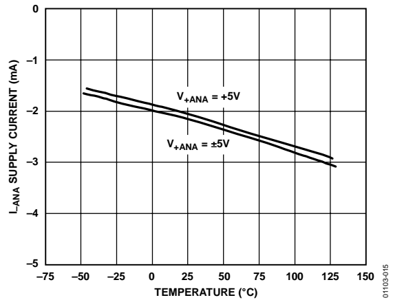
Figure 15. I_{-ANA} Supply Current/Comparator vs. Temperature
