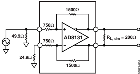
Figure 5. Basic Test Circuit
