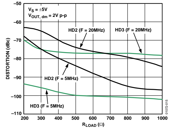
Figure 16. Harmonic Distortion vs. R LOAD
