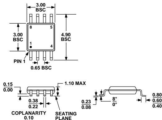
Figure 45. 8-Lead Mini Small Outline Package [MSOP] (RM-8)
