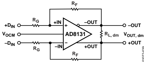
Figure 39. Circuit Definitions
