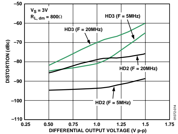
Figure 15. Harmonic Distortion vs. Differential Output Voltage
