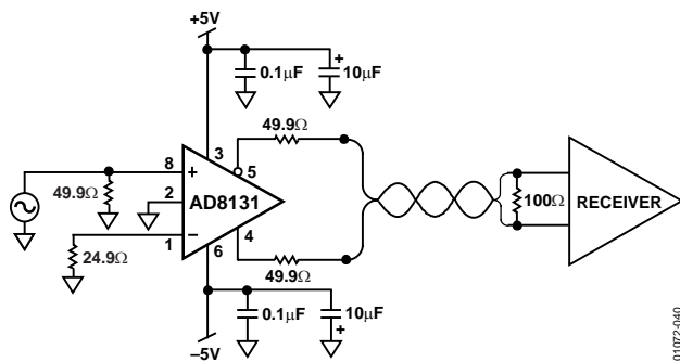
Figure 40. Single-Ended-to-Differential 100 Ω Line Driver
