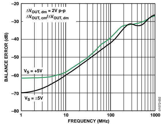
Figure 33. Output Balance Error vs. Frequency
