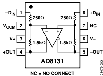
Figure 4. Pin Configuration
