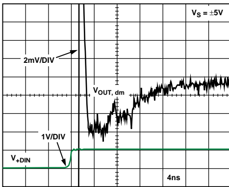
Figure 25. 0.1% Settling Time
