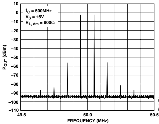
Figure 19. Intermodulation Distortion
