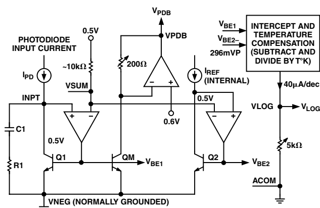
Figure 1. Simplified Schematic
