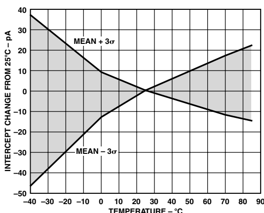
TPC 18. Intercept Drift vs. Temperature ( 3\sigma to Either Side of Mean)
