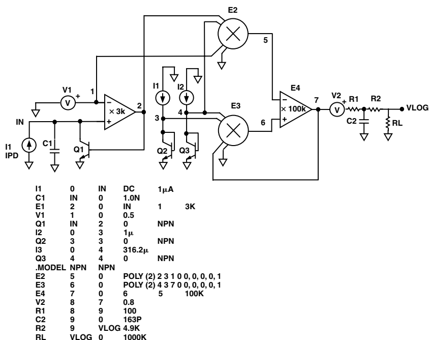
Figure 12. Basic Macromodel
