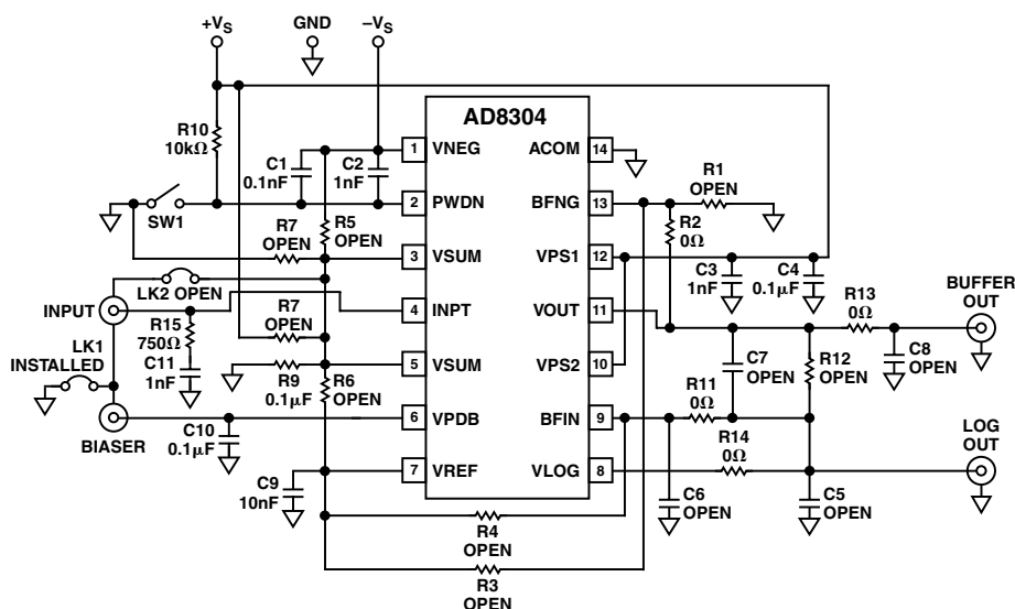
Figure 22. Evaluation Board Schematic
