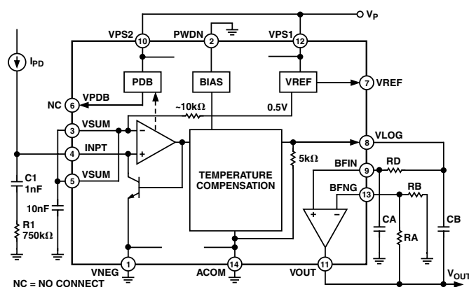
Figure 8. Two-Pole Low-Pass Filter
