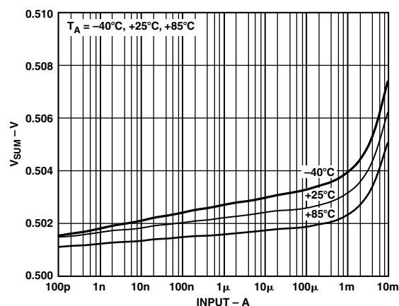
TPC 4. V_{SUM} vs. I_{PD}
