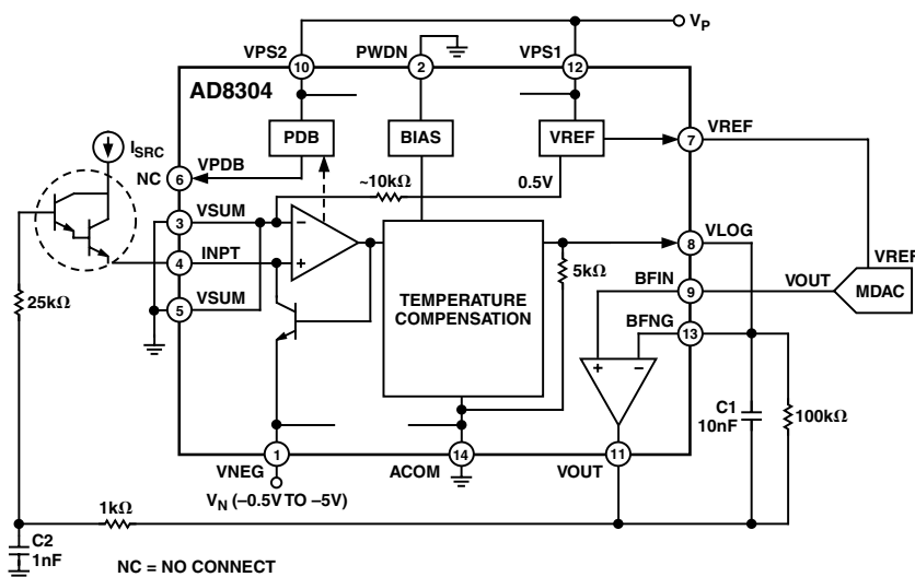
Figure 17. Multidecade Current Source
