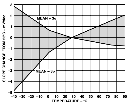
TPC 17. Slope Drift vs. Temperature ( 3\sigma to Either Side of Mean)
