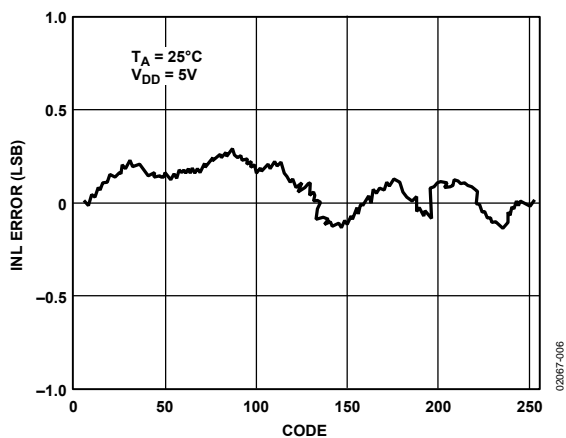
Figure 6. AD5307 INL
