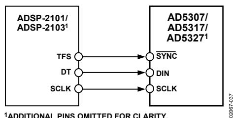
Figure 37. ADSP-2101/ADSP-2103-to-AD5307/AD5317/AD5327 Interface
