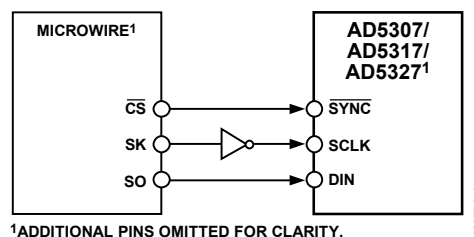
Figure 40. MICROWIRE-to-AD5307/AD5317/AD5327 Interface
