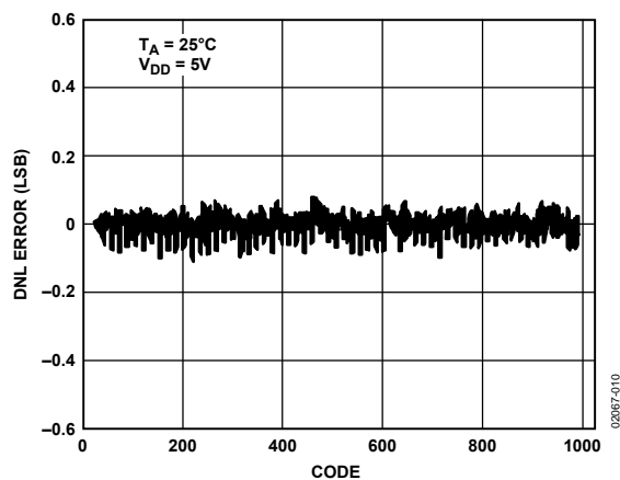
Figure 10. AD5317 DNL
