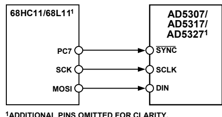
Figure 38. 68HC11/68L11-to-AD5307/AD5317/AD5327 Interface
