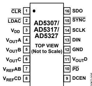
Figure 5. Pin Configuration
