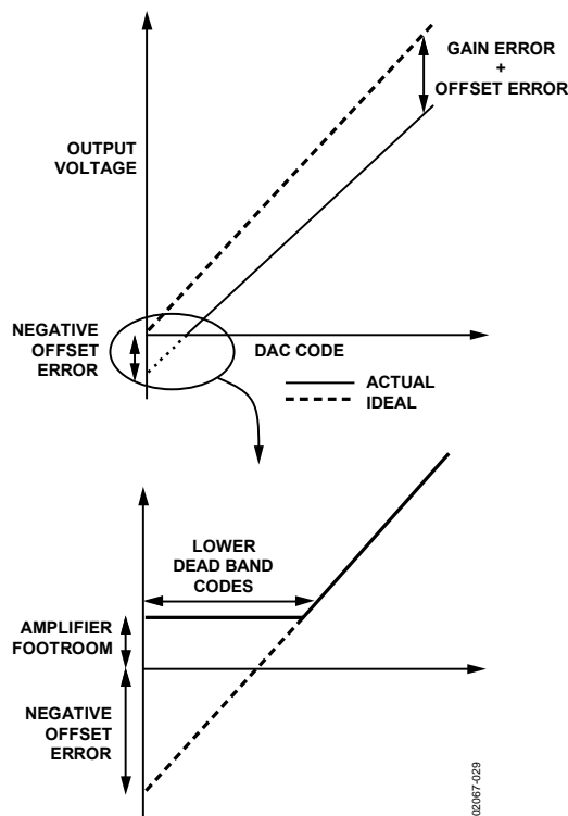
Figure 29. Transfer Function with Negative Offset
