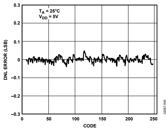
Figure 9. AD5307 DNL
