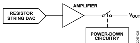
Figure 36. Output Stage During Power-Down
