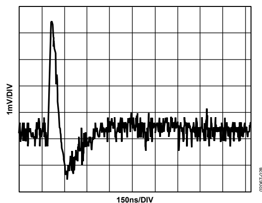
Figure 28. DAC-to-DAC Crosstalk
