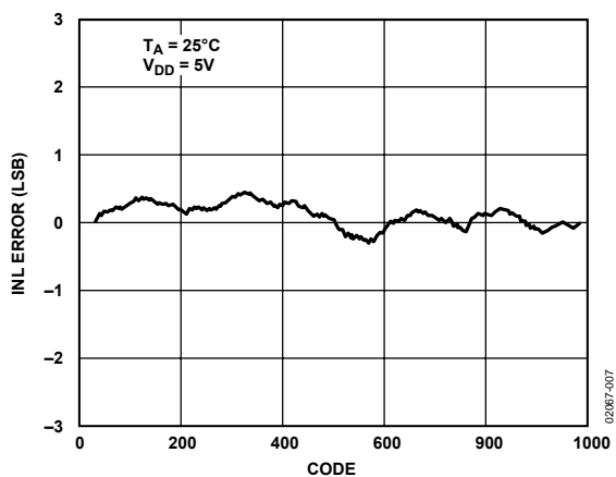
Figure 7. AD5317 INL
