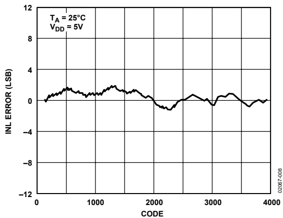
Figure 8. AD5327 INL
