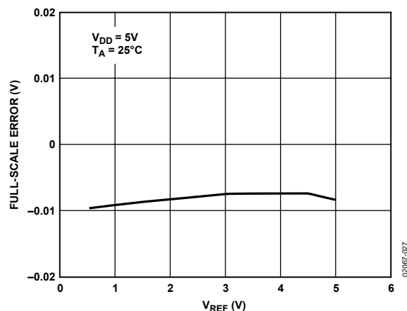
Figure 27. Full-Scale Error vs. V_{REF}
