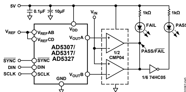
Figure 45. Window Detection
