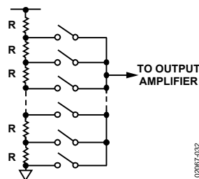
Figure 32. Resistor String
