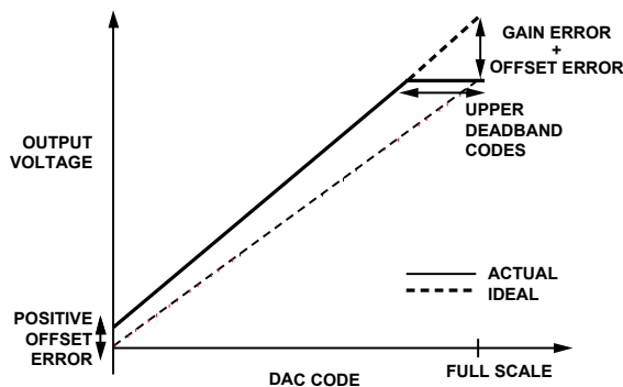
Figure 30. Transfer Function with Positive Offset ( V_{REF} = V_{DD} )
