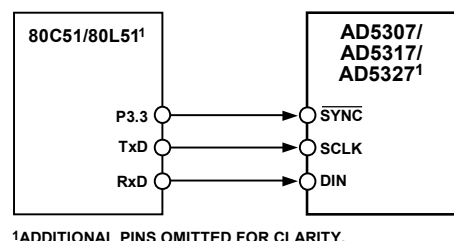
Figure 39. 80C51/80L51-to-AD5307/AD5317/AD5327 Interface
