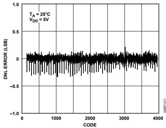
Figure 11. AD5327 DNL
