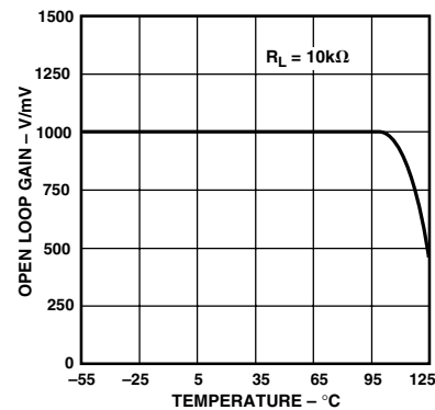
TPC 9. Open-Loop Gain vs. Temperature
