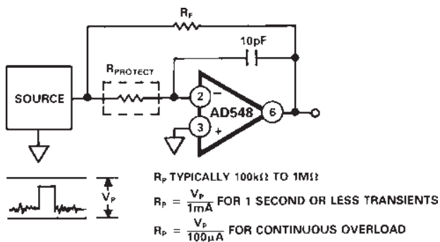
Figure 3. Input Protection of IV Converter
