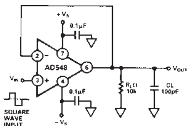
TPC 19a. Unity Gain Follower
