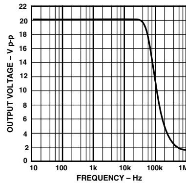
TPC 14. Large Signal Frequency Response
