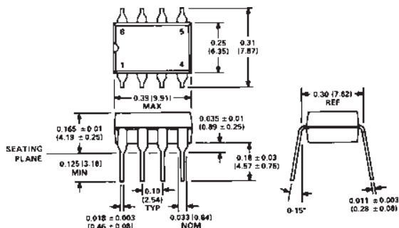
Plastic Mini-DIP (N) Package Dimensions shown in inches and (millimeters)
