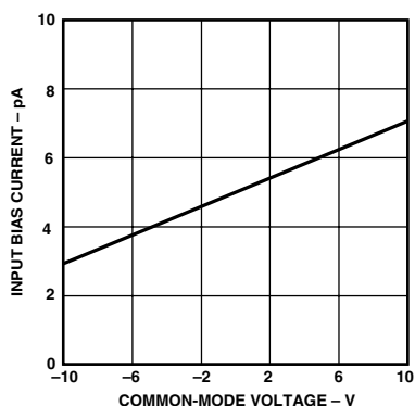
TPC 7. Input Bias Current vs. Common-Mode Voltage
