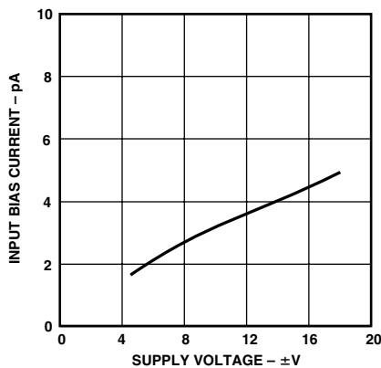
TPC 5. Input Bias Current vs. Supply Voltage
