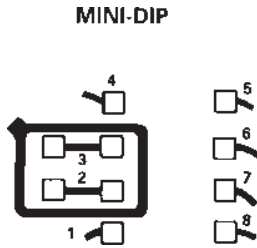
Figure 2. Board Layout for Guarding Inputs
