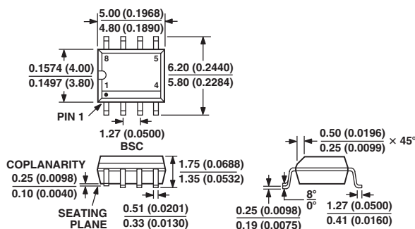
SOIC (R) Package Dimensions shown in millimeters and (inches)
