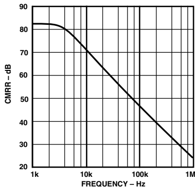
TPC 13. CMRR vs. Frequency
