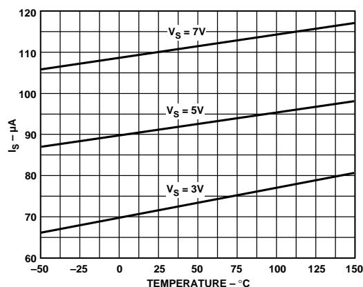
Figure 8. Supply Current vs. Temperature ( V_{OUT} = \text{LOW} )
