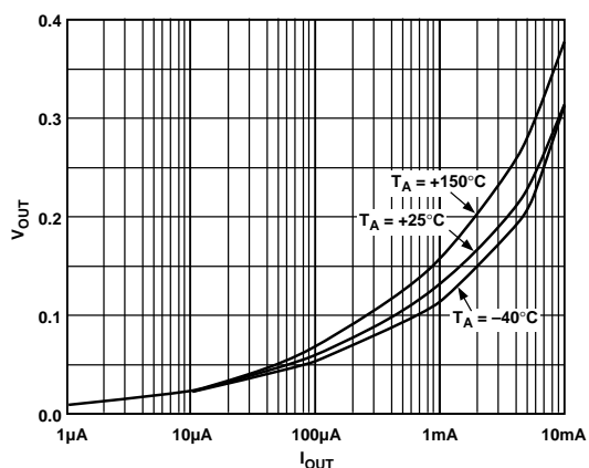
Figure 9. V_{OUT} vs. I_{OUT} ( V_{OUT} = LOW )
