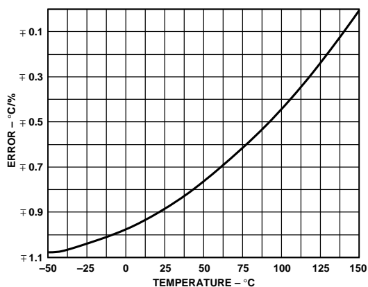
Figure 4. Setpoint Error Due to R_{SET} Tolerance
