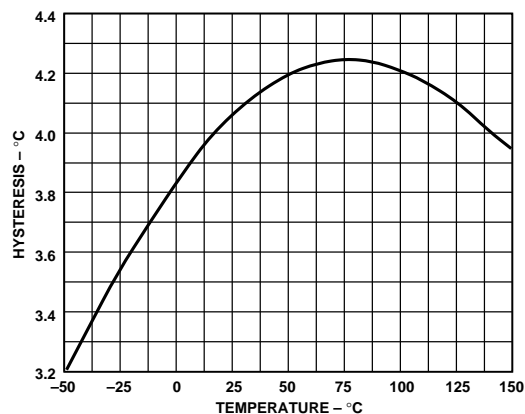
Figure 6. Hysteresis vs. Setpoint
