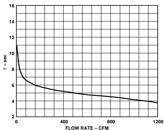
Figure 10. Thermal Response vs. Flow Rate
