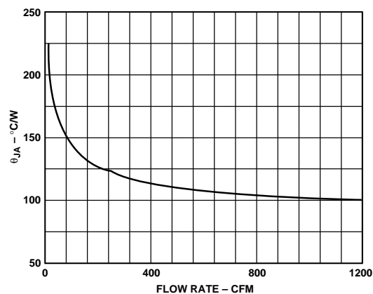
Figure 11. Thermal Resistance vs. Flow Rate
