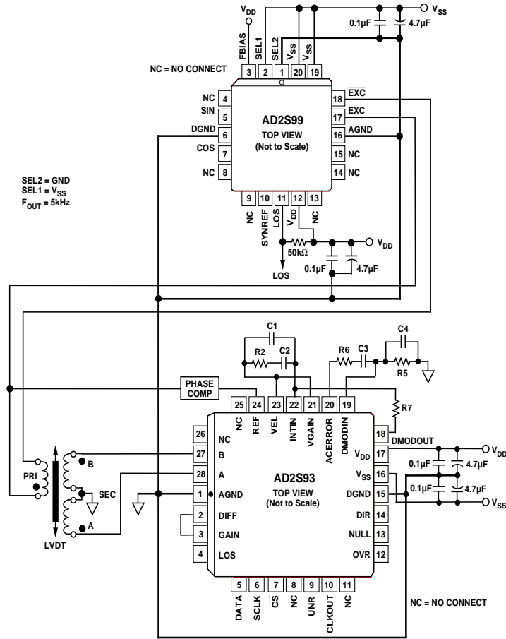
Figure 5. AD2S99 and AD2S93 Example Configuration
