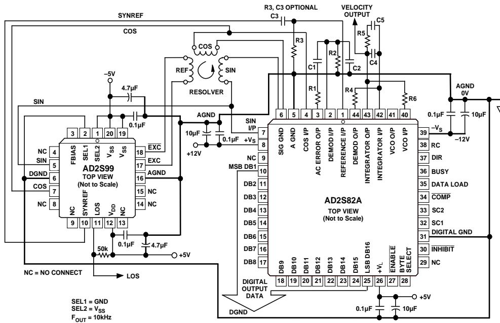
Figure 4. AD2S99 and AD2S82A Example Configuration
