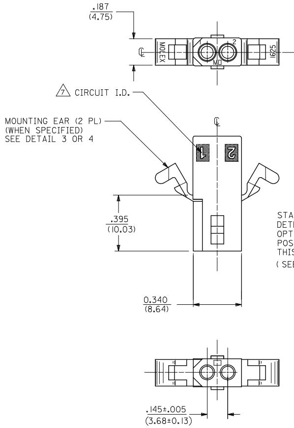
OPTIONAL POSITIVE LOCK ONE SIDE ONLY SCALE 4:1
