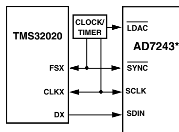
Figure 13. AD7243-TMS32020 Interface
