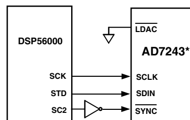
Figure 12. AD7243-DSP56000 Interface
