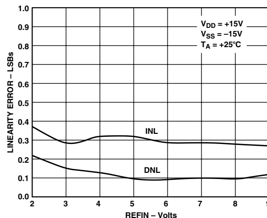
Figure 4. Typical Linearity vs. REF IN Voltage
