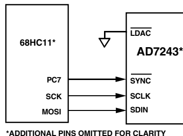
Figure 15. AD7243–68HC11 Interface
