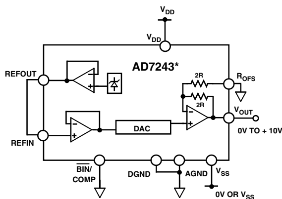
Figure 9. Unipolar (0 V to +10 V) Configuration
