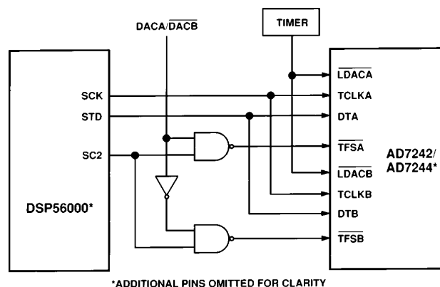
Figure 8. AD7242/AD7244 to DSP56000 Interface
