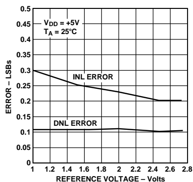
Figure 6. Relative Accuracy vs. External Reference
