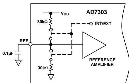
Figure 21. Reference Input
