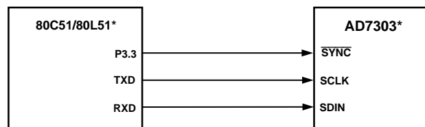
Figure 28. AD7303 to 80C51/80L51 Interface
