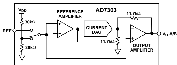
Figure 20. DAC Architecture
