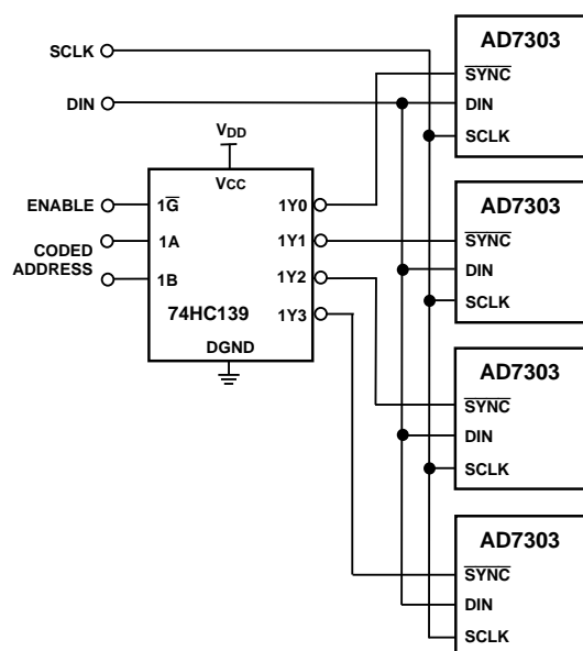
Figure 33. Decoding Multiple AD7303 Devices in a System
