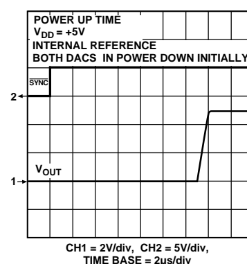
Figure 11. Exiting Power-Down (Full Power-Down)
