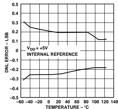
Figure 17. Typical DNL vs. Temperature
