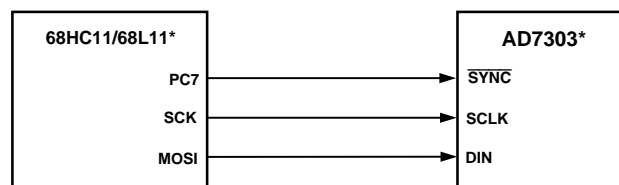
Figure 27. AD7303 to 68HC11/68L11 Interface
