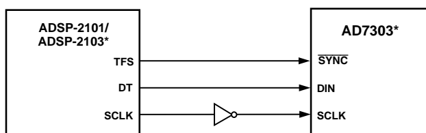
Figure 26. AD7303 to ADSP-2101/ADSP-2103 Interface
