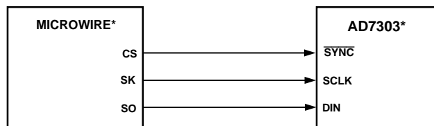
Figure 29. AD7303 to Microwire Interface
