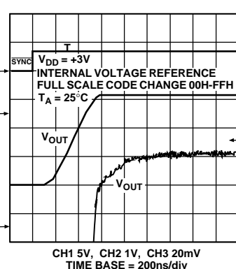
Figure 10. Full-Scale Settling Time
