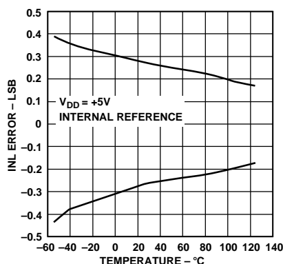
Figure 16. Typical INL vs. Temperature
