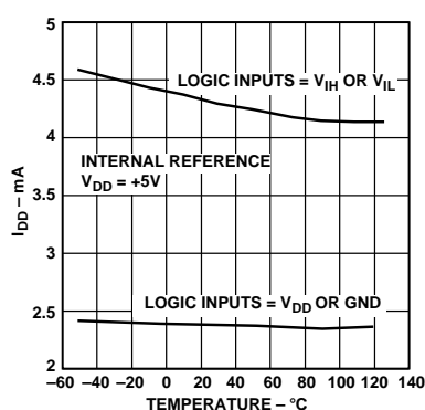
Figure 7. Supply Current vs. Temperature
