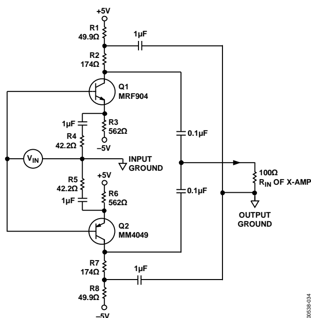
Figure 36. A Low Noise Preamplifier for the AD600/AD602
