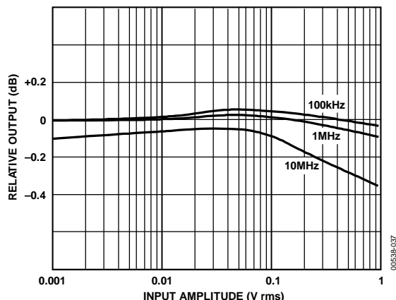
Figure 39. Output Stabilization vs. rms Input for Sine Wave Inputs at 100 kHz, 1 MHz, and 10 MHz
