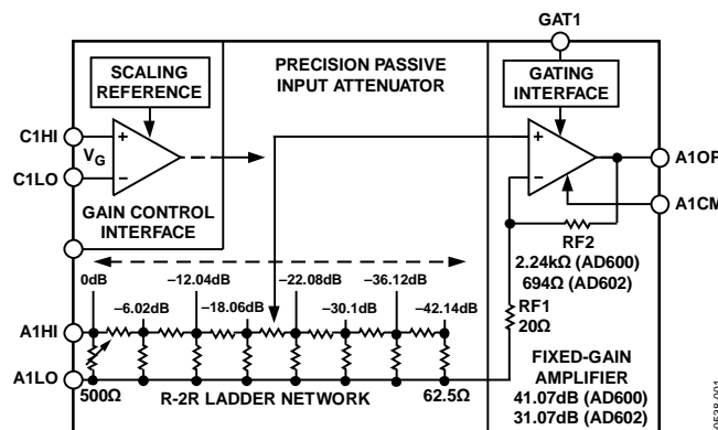
Figure 1. Functional Block Diagram of a Single Channel of the AD600/AD602
