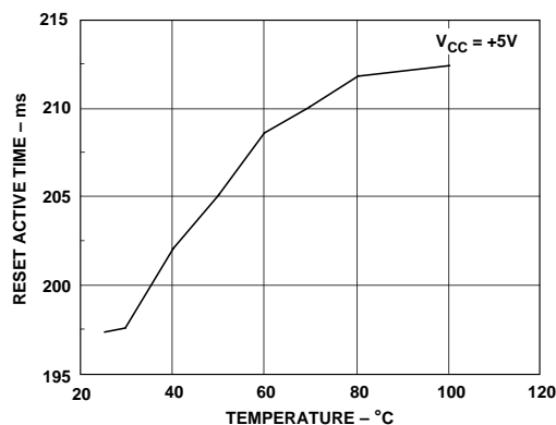
Figure 2. \overline{RESET} Active Time vs. Temperature
