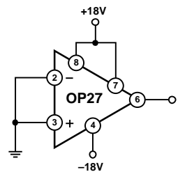
Figure 45. Burn-In Circuit
