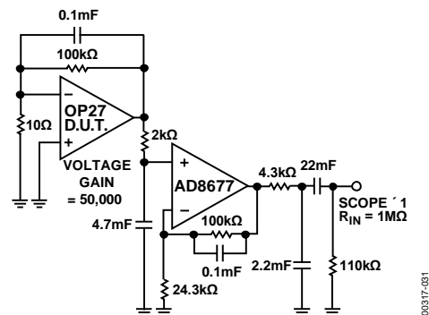
Figure 31. Voltage Noise Test Circuit (0.1 Hz to 10 Hz)
