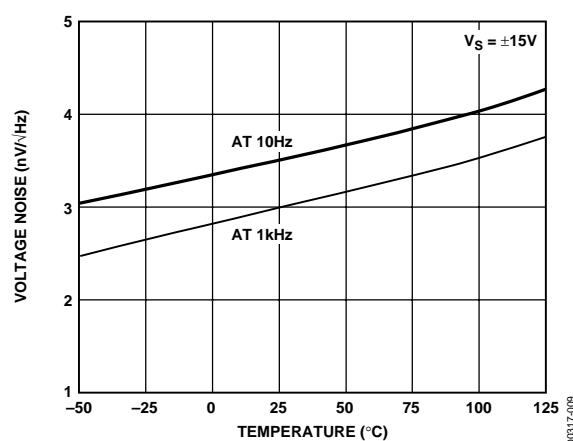
Figure 9. Voltage Noise Density vs. Temperature
