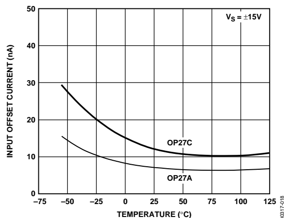
Figure 18. Input Offset Current vs. Temperature
