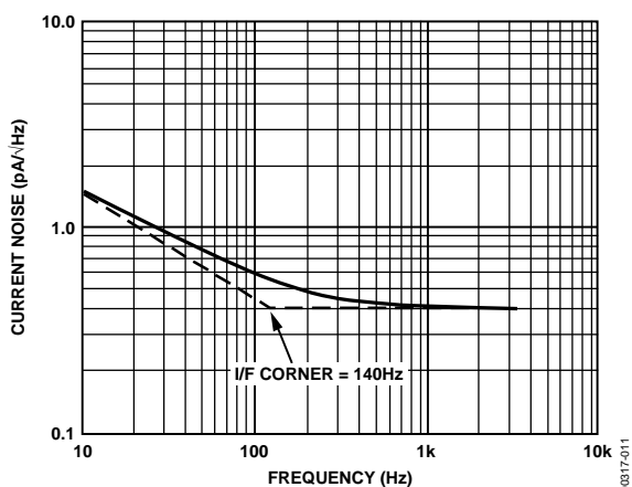
Figure 11. Current Noise Density vs. Frequency
