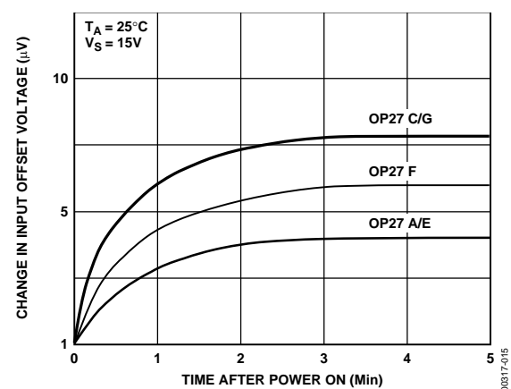
Figure 15. Warm-Up Offset Voltage Drift
