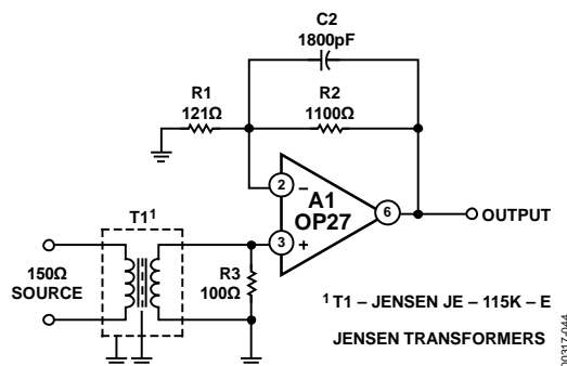
Figure 44. High Quality Microphone Transformer Coupled Preamplifier
