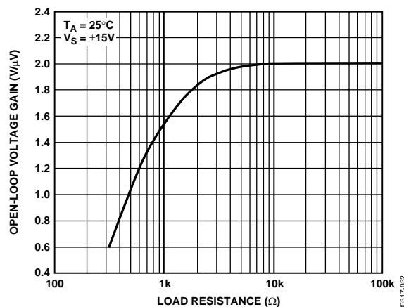
Figure 32. Open-Loop Voltage Gain vs. Load Resistance
