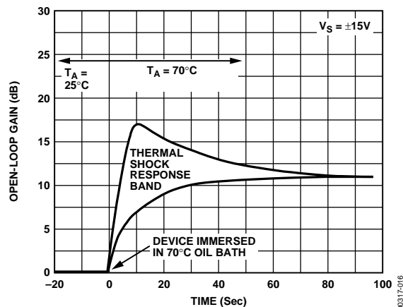
Figure 16. Offset Voltage Change Due to Thermal Shock
