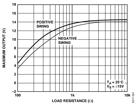
Figure 24. Maximum Output Voltage vs. Load Resistance
