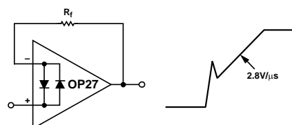
Figure 37. Pulsed Operation
