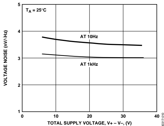
Figure 10. Voltage Noise Density vs. Supply Voltage
