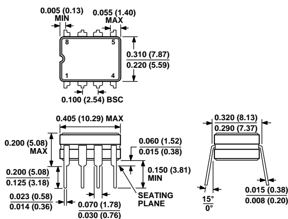
Figure 47. 8-Lead Ceramic DIP - Glass Hermetic Seal [CERDIP] (Q-8) Z-Suffix Dimensions shown in inches and (millimeters)
