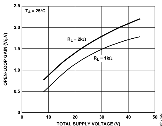
Figure 22. Open-Loop Voltage Gain vs. Supply Voltage
