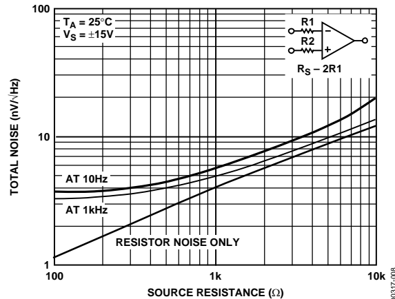
Figure 8. Total Noise vs. Sourced Resistance
