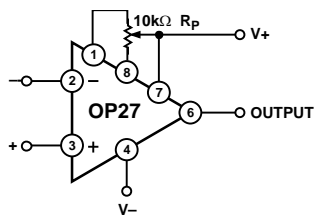
Figure 35. Offset Nulling Circuit
