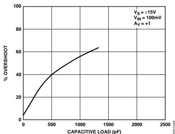
Figure 25. Small-Signal Overshoot vs. Capacitive Load
