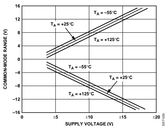
Figure 30. Common-Mode Input Range vs. Supply Voltage
