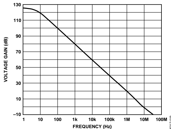
Figure 19. Open-Loop Gain vs. Frequency
