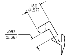
DETAIL 4 .093/(2.36) PREBENT MOUNTING EAR (SCALE 4:1)
