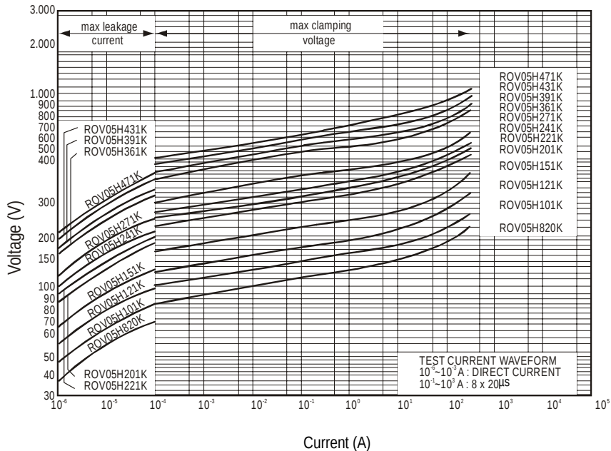
ROV05H820K – ROV05H471K
