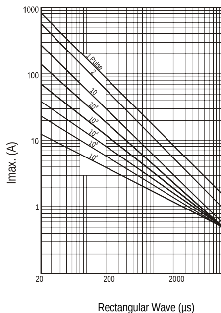
ROV05H820K – ROV05H471K
