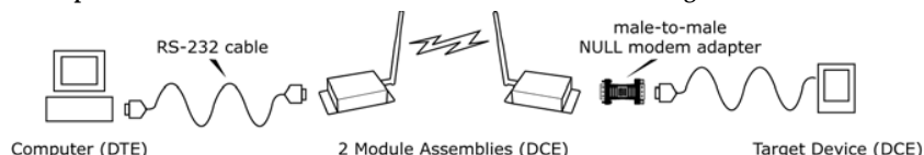
Figure B-06. Example of a MaxStream Radio Modem (DCE Device) connecting to another DCE device
