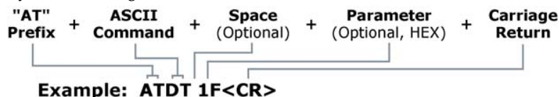
Figure 2-09. Syntax for sending AT Commands
