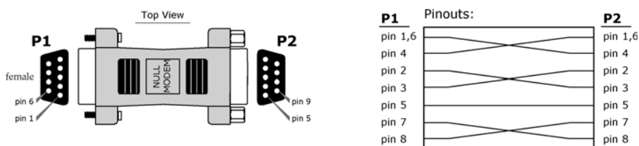
Figure B-07. Female NULL modem adapter and pinouts
