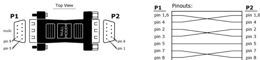
Figure B-06. Example of a MaxStream Radio Modem (DCE Device) connecting to another DCE device
