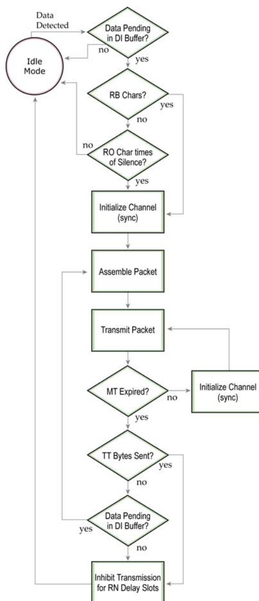
Figure 4-05. Multi-Transmit Mode State Diagram (TX Module)
