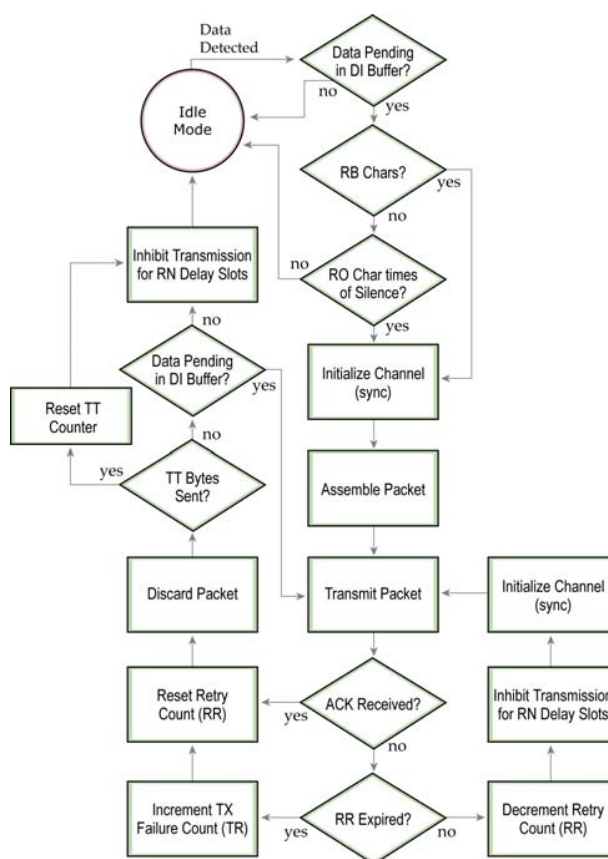
Figure 4-07. Acknowledged Mode State Diagram (TX module)
