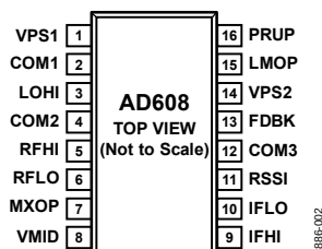
Figure 2. Pin Configuration
