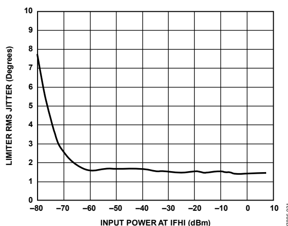
Figure 13. Limiter RMS Jitter Performance vs. Input Power at IFHI (See Figure 21)
