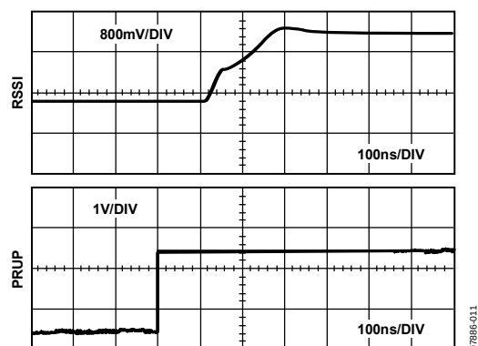
Figure 8. RSSI Power-Up Response (See Figure 19)
