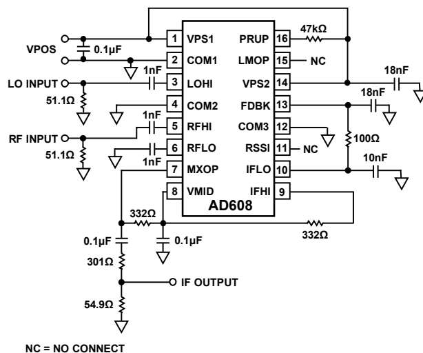
Figure 18. Mixer Test Board Schematic
