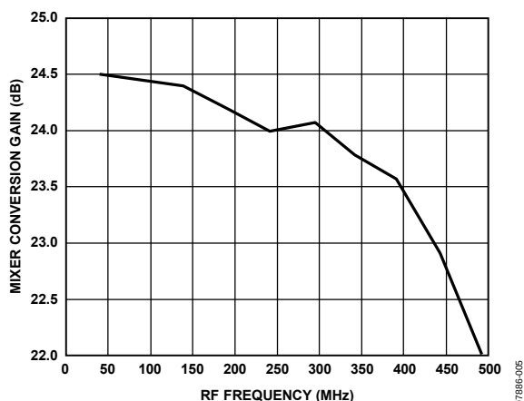
Figure 3. Mixer Conversion Gain vs. RF Frequency
