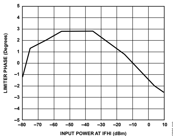
Figure 12. Limiter Phase Performance vs. Input Power at IFHI (See Figure 21)
