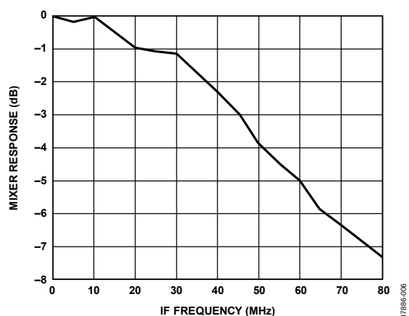
Figure 4. Mixer IF Port Bandwidth
