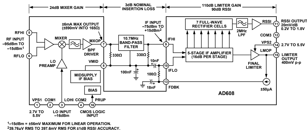
Figure 22. Functional Block Diagram
