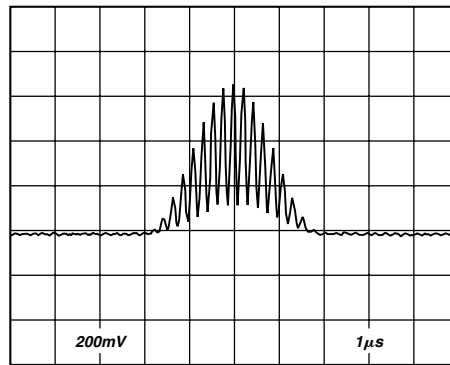
TPC 9. Zoom on Modulated Pulse, PAL
