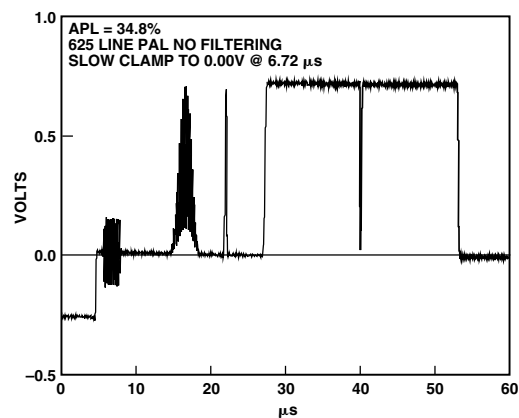
TPC 8. Modulated Pulse and Bar, PAL
