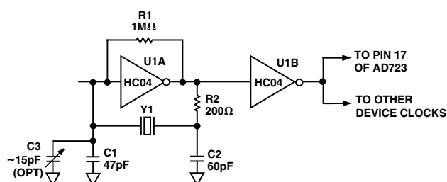
Figure 9. Low Cost Crystal Oscillator
