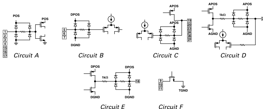
Figure 1. Equivalent Circuits
