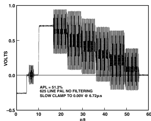
TPC 4. 100% Color Bars, PAL
