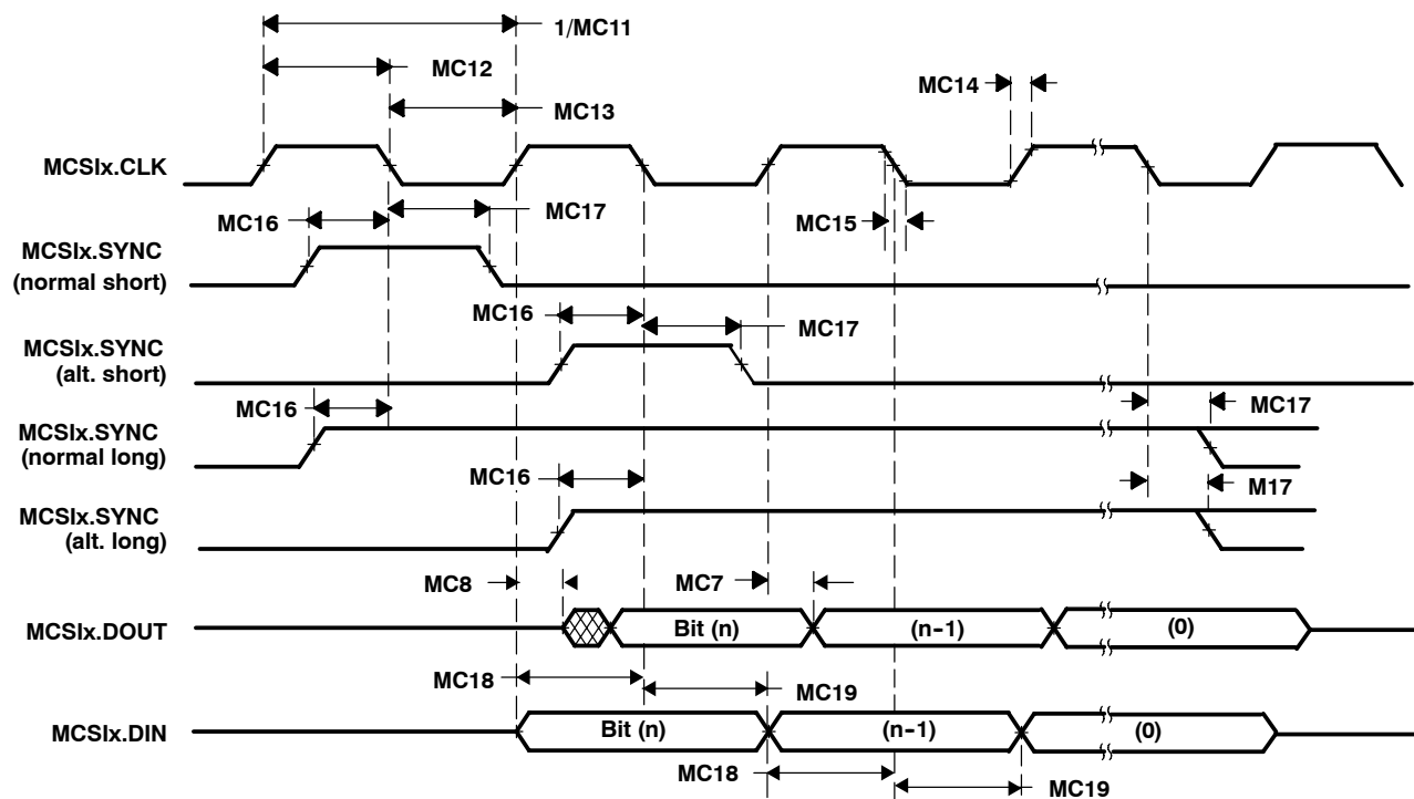
Figure 5-25. MCSI Slave Mode Timings
