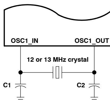
Figure 5-4. Internal System Oscillator External Crystal
