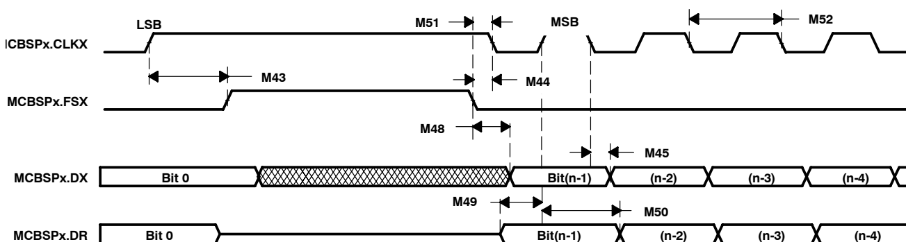
Figure 5-22. McBSP Timing as SPI Master or Slave: CLKSTP = 10b, CLKXP = 1
