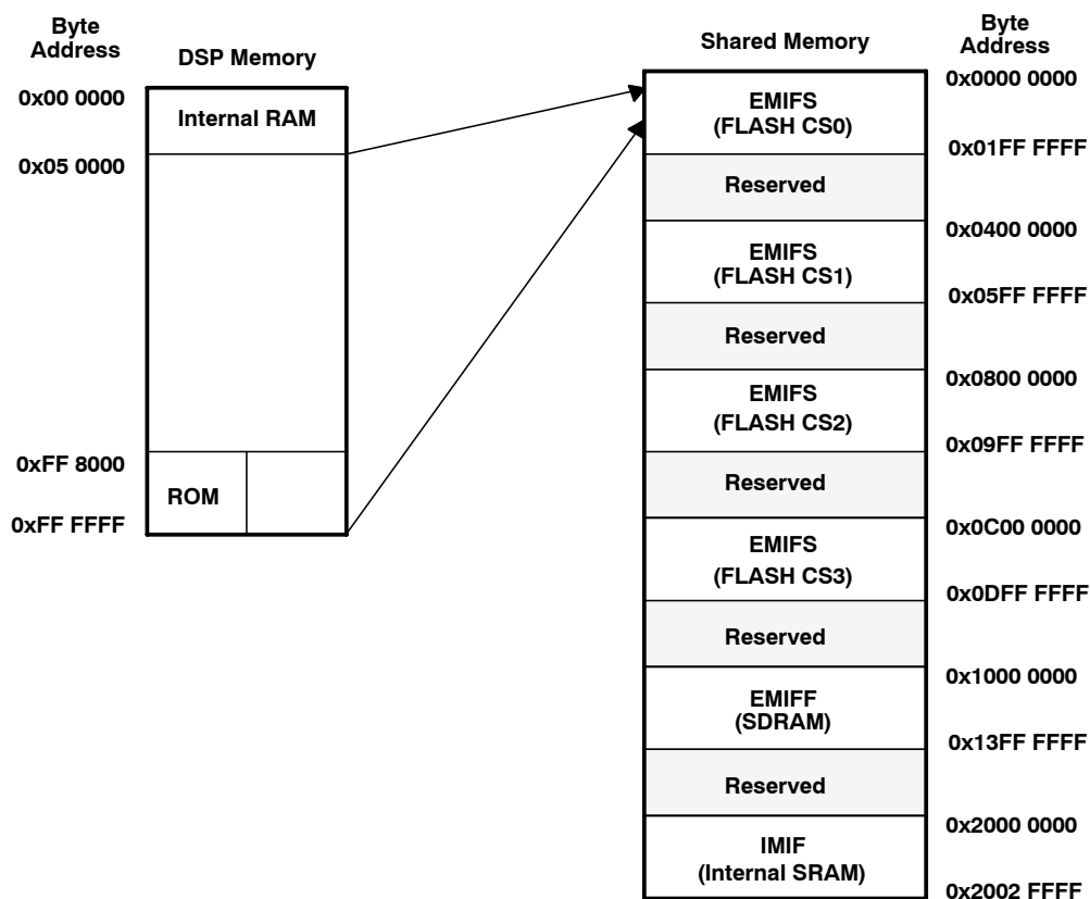
Figure 3-2. DSP MMU Off
