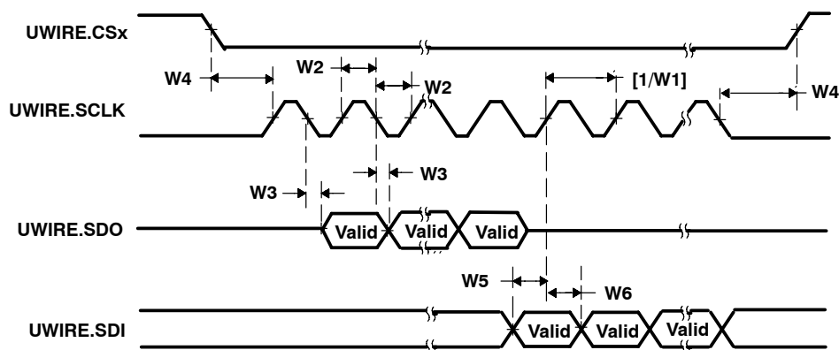
Figure 5-35. MICROWIRE Timings
