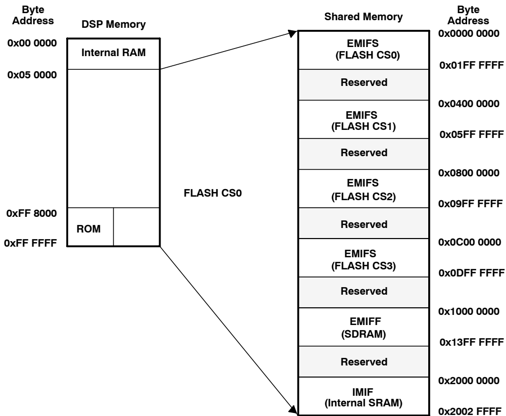
Figure 3-3. DSP MMU On
