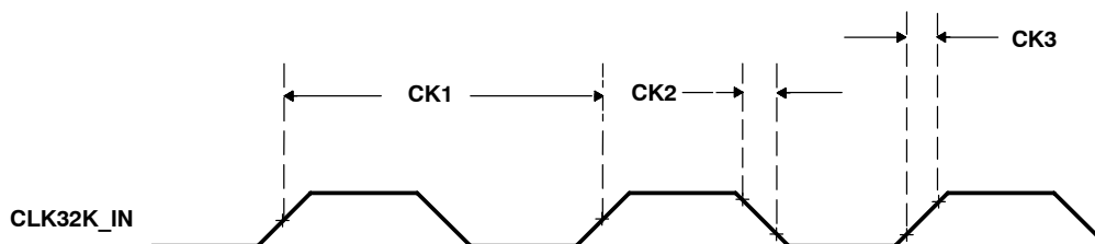
Figure 5-3. 32-kHz Input Clock
