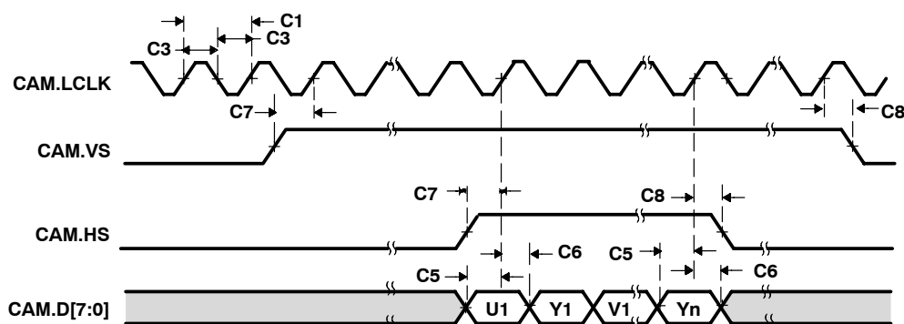
Figure 5-26. Camera Interface Timings
