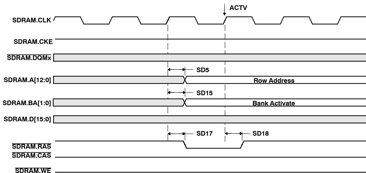
Figure 5-14. SDRAM ACTV (Activate Row) Command
