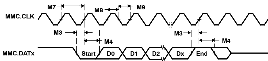
Figure 5-32. MMC/SD Host Read and Card CRC Status Timings
