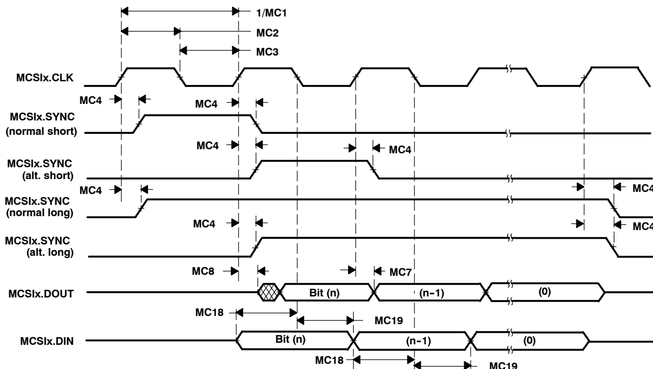
Figure 5-24. MCSI Master Mode Timings
