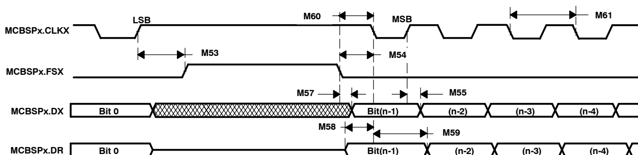
Figure 5-23. McBSP Timing as SPI Master or Slave: CLKSTP = 11b, CLKXP = 1
