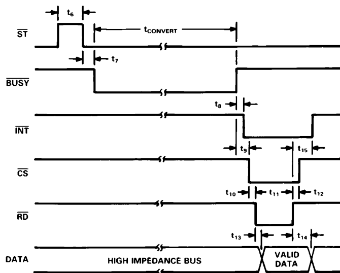
Figure 10. ADC Mode 1 Interface Timing
