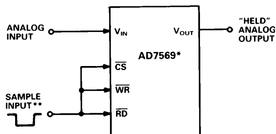
Figure 29. Infinite Sample-and-Hold
