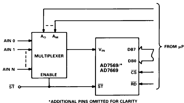
Figure 11. Multichannel Inputs
