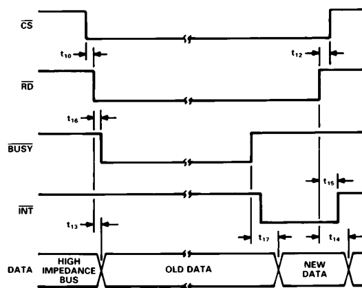
Figure 12. ADC Mode 2 Interface Timing
