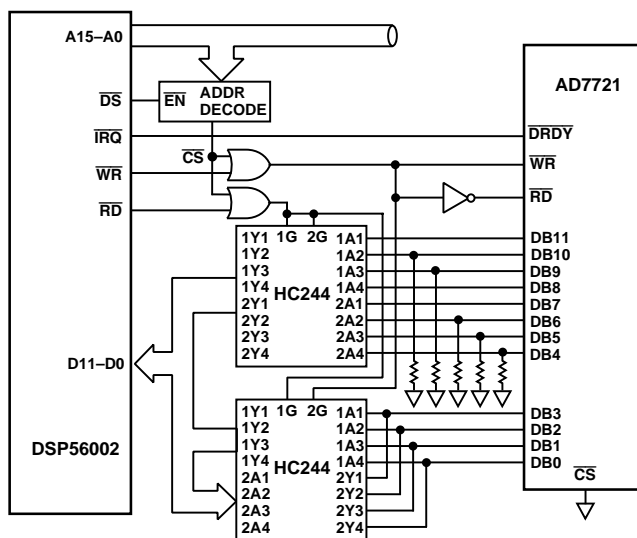
Figure 18. AD7721 to DSP56002 Interface
