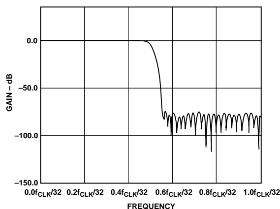
Figure 9b. 83 Tap FIR Filter Frequency Response
