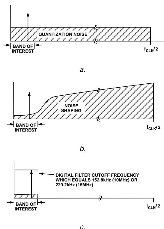
Figure 8. Sigma-Delta ADC
