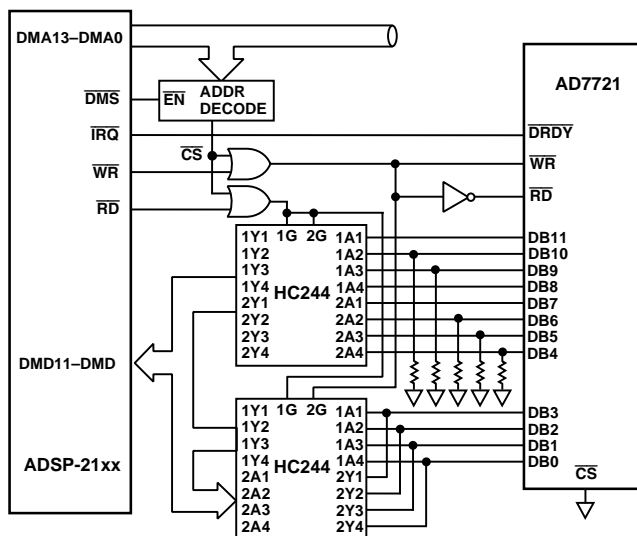
Figure 17. AD7721 to ADSP-21xx Interface
