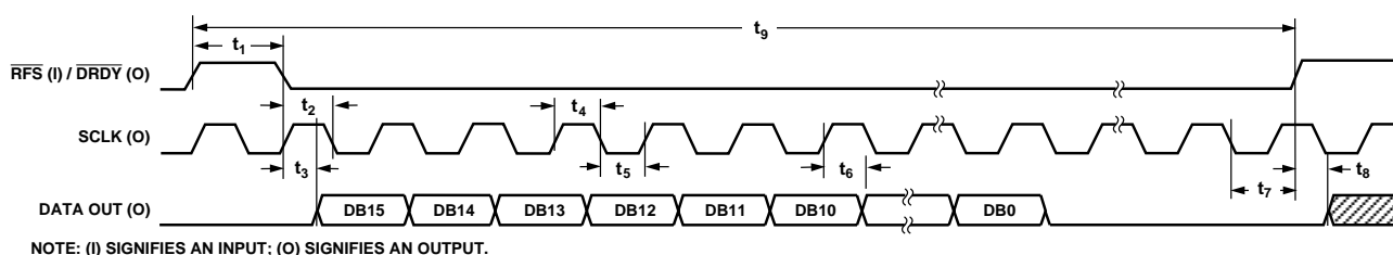
Figure 10. Serial Mode Output Register Read
