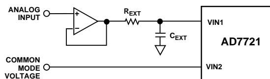
Figure 6. Antialiasing Circuits
