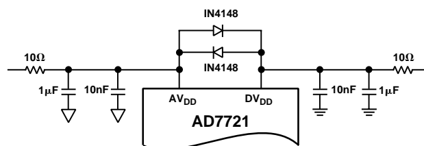
Figure 7. Powering-Up Protection Scheme
