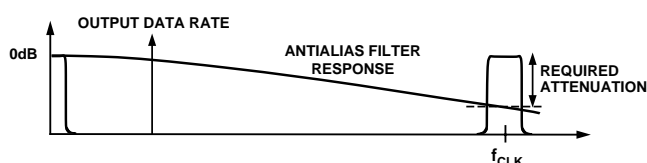
b. Frequency Response of Antialias Filter (AD7721)
