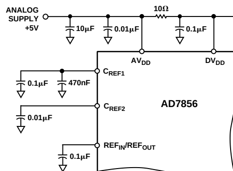
Figure 16. Relevant Connections When Using Internal Reference
