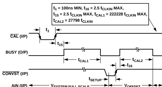
Figure 29. Timing Diagram for Full System Calibration
