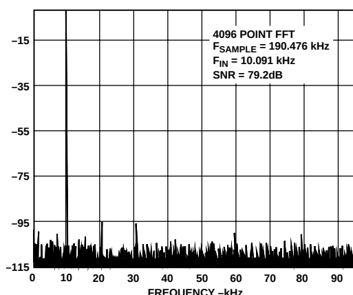
Figure 18. FFT Plot
