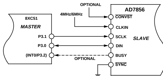
Figure 37. 8XC51/PIC16C42 Interface
