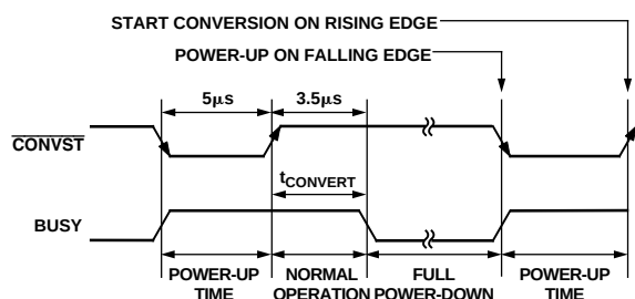
Figure 22. Power-Up Timing When Using \overline{\text{CONVST}} Pin
