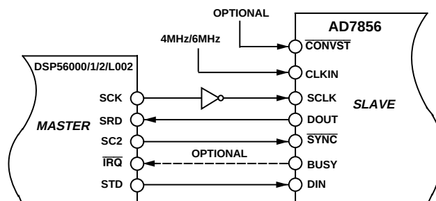
Figure 40. DSP56000/1/2/L002 Interface
