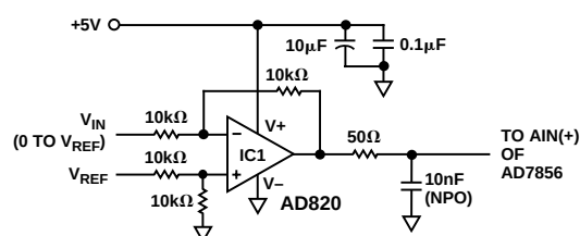
Figure 13. Analog Input Buffering
