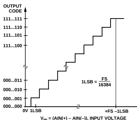
Figure 15. Transfer Characteristic
