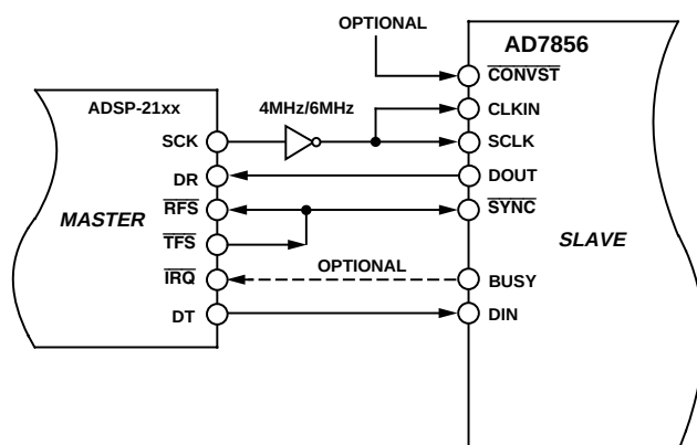
Figure 39. ADSP-21xx Interface
