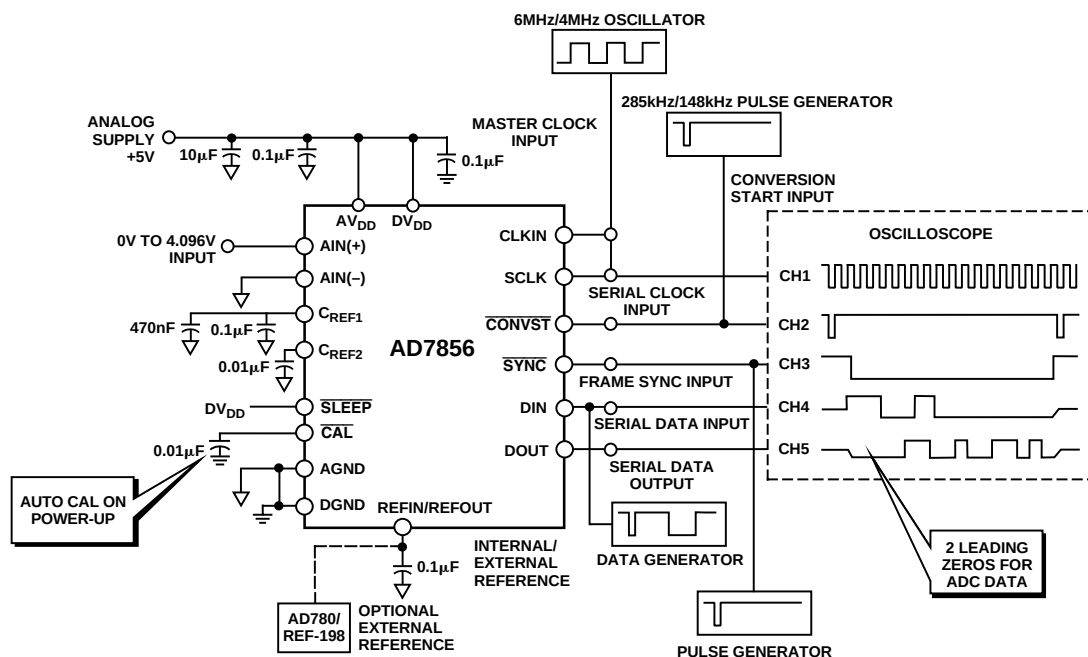
Figure 10. Typical Circuit
