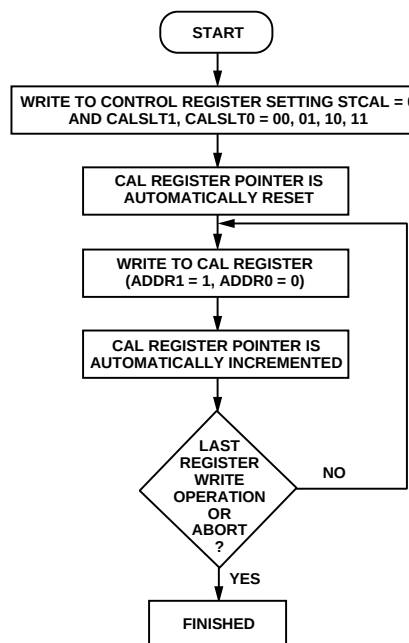
Figure 8. Flowchart for Writing to the Calibration Registers
