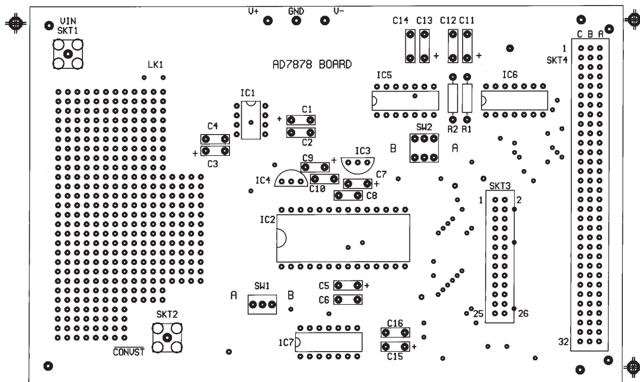
Figure 24. PCB Silkscreen for Figure 23
