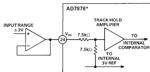
Figure 15. AD7878 Analog Input
