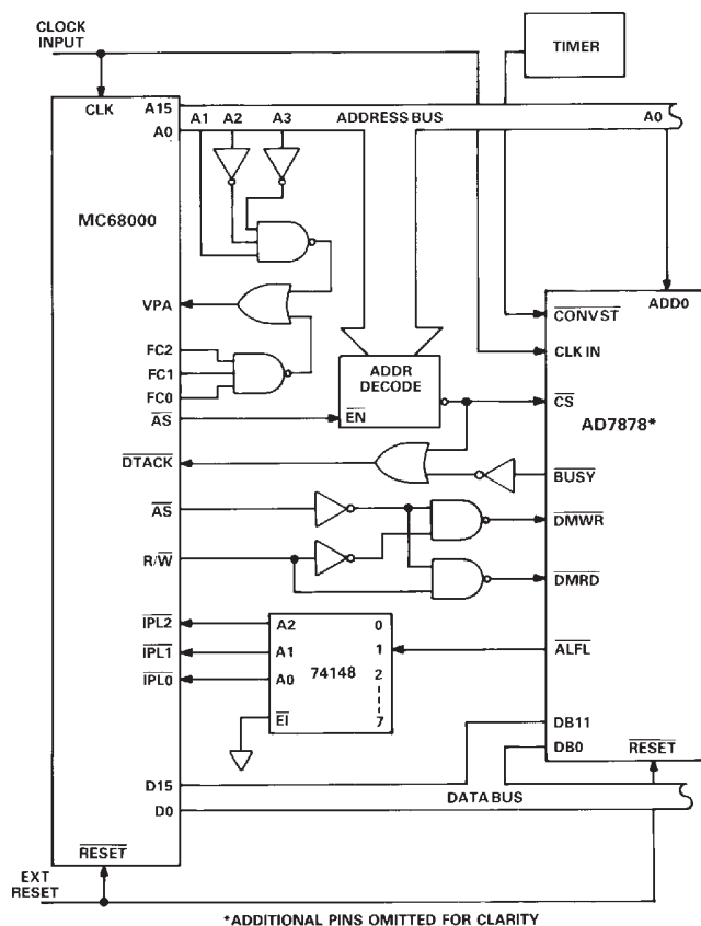
Figure 21. AD7878–MC68000 Interface
