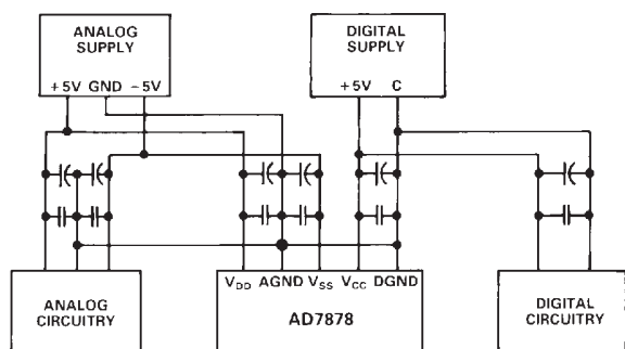
Figure 22. Power Supply Grounding Practice
