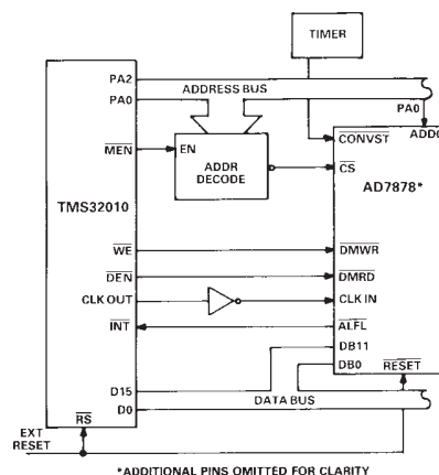
Figure 20. AD7878-TMS32010 Interface
