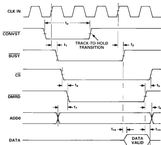
Figure 9. Extended Read Operation
