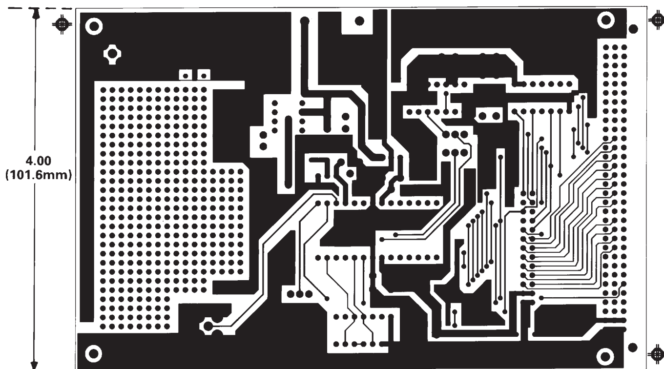
Figure 25. PCB Component Side Layout for Figure 23
