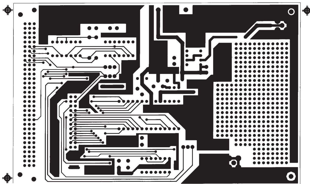
Figure 26. PCB Solder Side Layout for Figure 23
