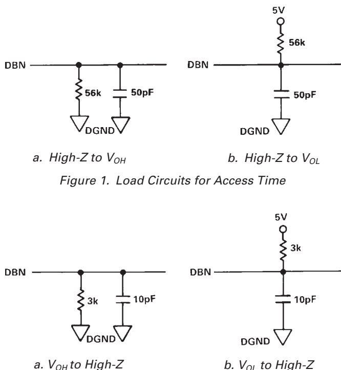
Figure 2. Load Circuits for Output Float Delay
