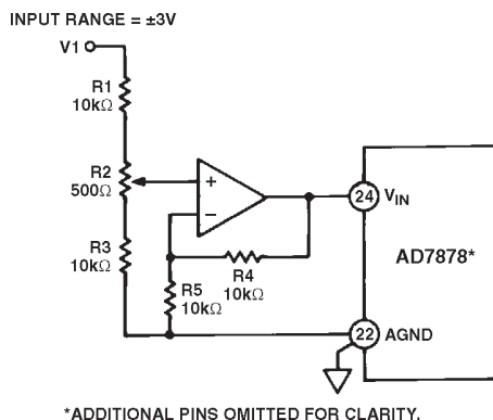
Figure 17. AD7878 Full-Scale Adjust Circuit
