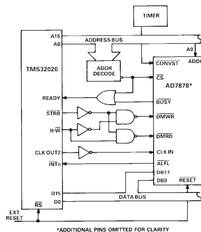
Figure 19. AD7878-TMS32020 Interface
