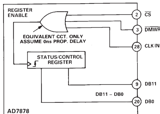
Figure 7. \overline{DMWR} Internal Logic
