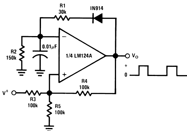
Figure 26. Pulse Generator
