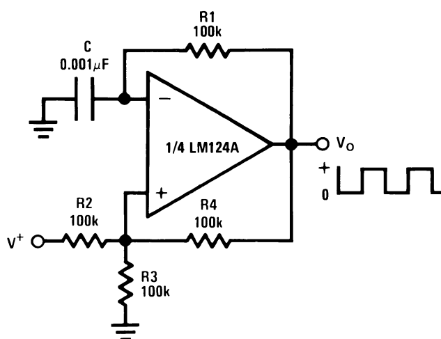
Figure 27. Squarewave Oscillator
