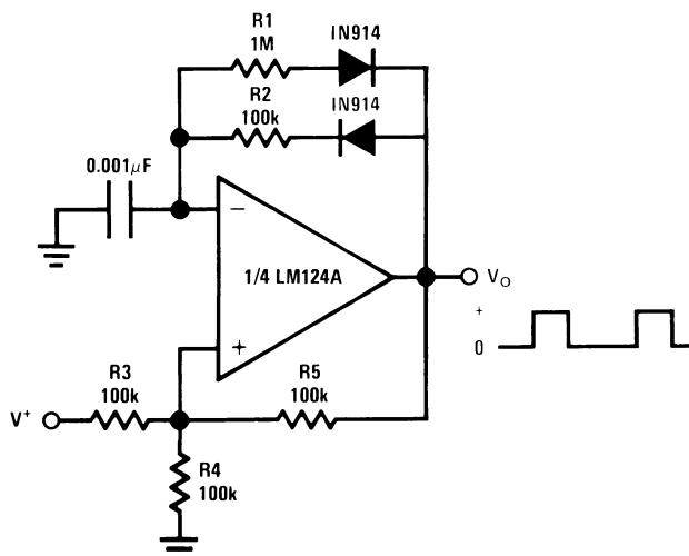
Figure 26. Pulse Generator
