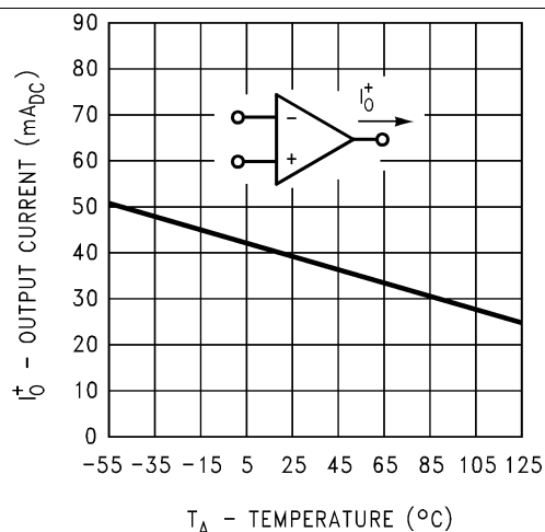
Figure 12. Current Limiting
