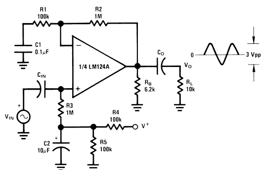
Figure 36. AC Coupled Inverting Amplifier
