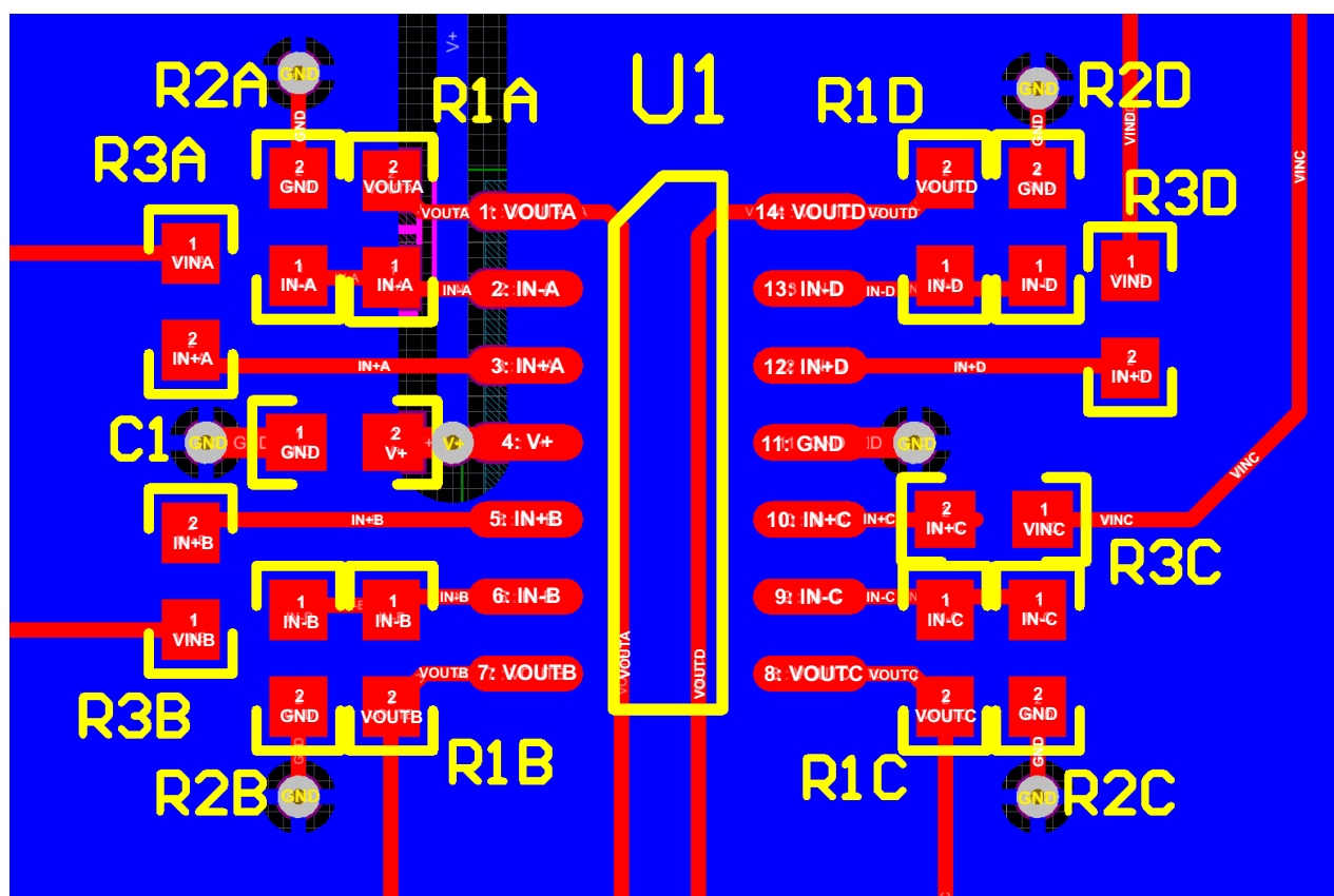
Figure 43. Layout Example
