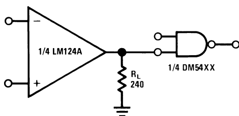
Figure 24. Driving TTL
