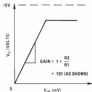
Figure 16. Non-Inverting Amplified Response Curve
