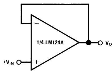
Figure 25. Voltage Follower
