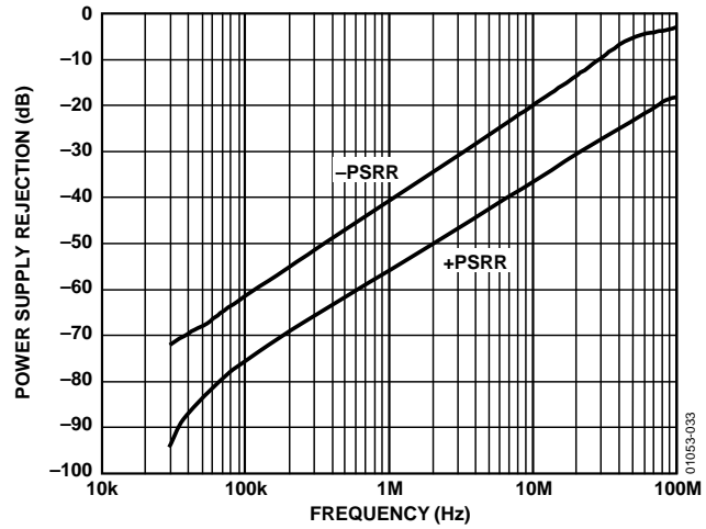
Figure 33. Power Supply Rejection vs. Frequency VS = ±12 V
