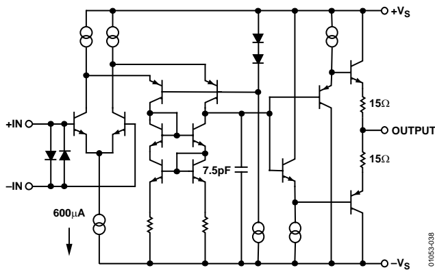
Figure 38. Simplified Schematic
