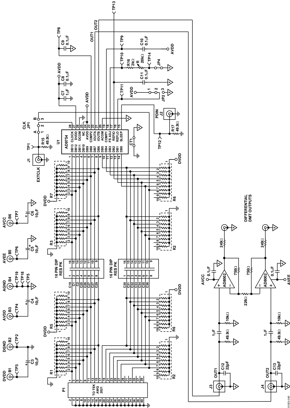
Figure 40. DMT Signal Generator Schematic
