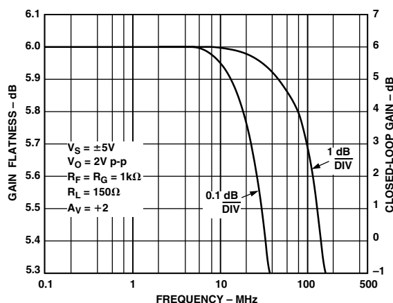
Figure 1. Large Signal Frequency Response
