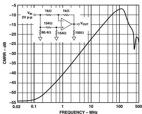
TPC 17. CMRR vs. Frequency; V_S = \pm 5V
