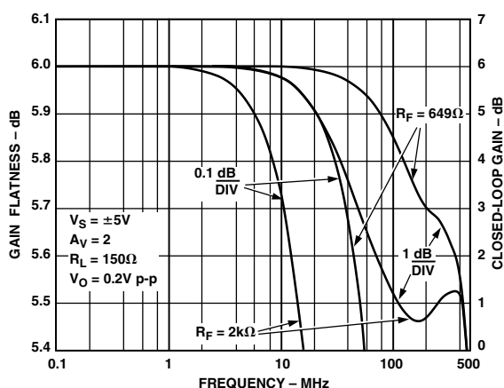
Figure 5. Frequency Response vs. R_F
