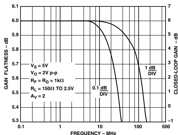
TPC 12. Large Signal Frequency Response
