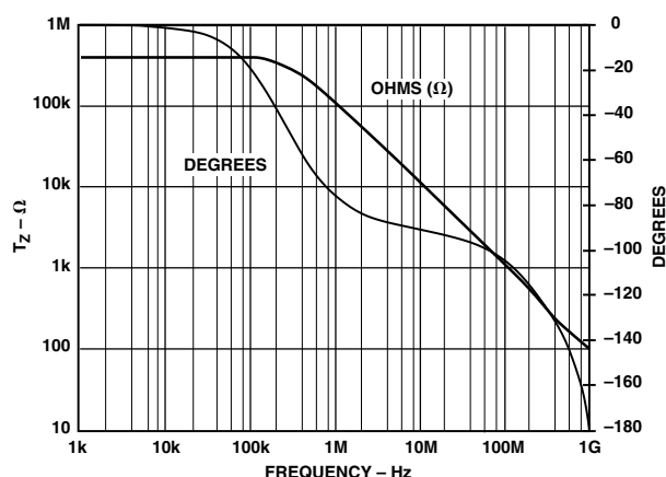
TPC 10. Open-Loop Transimpedance vs. Frequency
