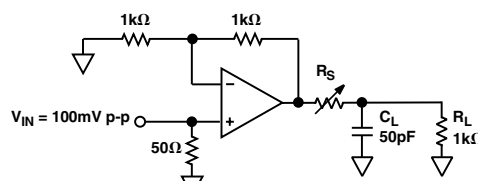
Figure 7. Capacitive Load Drive Circuit
