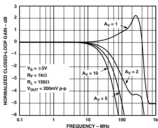
TPC 11. Normalized Frequency Response; V_S = \pm 5 V
