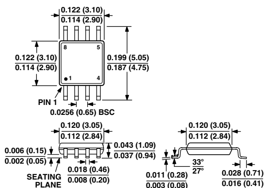
8-Lead \mu SOIC (RM-8)
