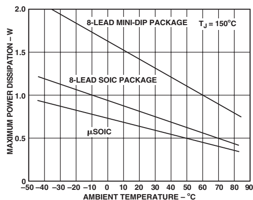
Figure 2. AD8072 Maximum Power Dissipation vs. Temperature
