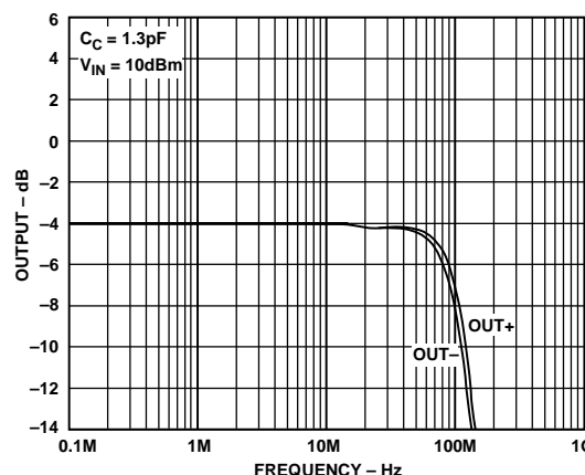
Figure 28. Differential Driver Frequency Response
