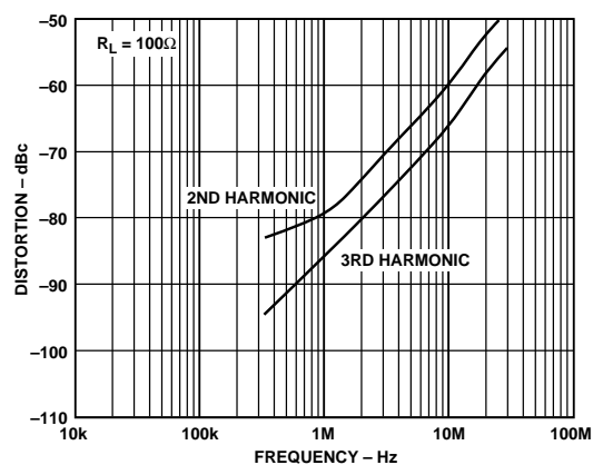
Figure 7. Distortion vs. Frequency, R_L = 100\ \Omega
