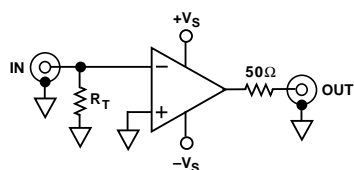
Inverting Configuration
