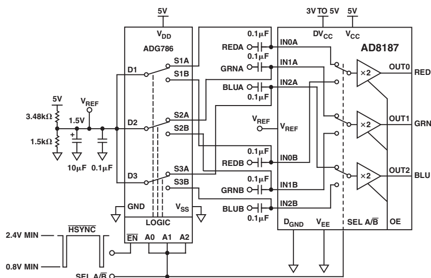
Figure 11. AD8187 AC-Coupled with DC Restore
