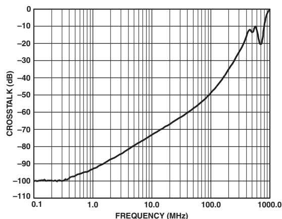
TPC 10. AD8187 All Hostile Crosstalk* vs. Frequency
