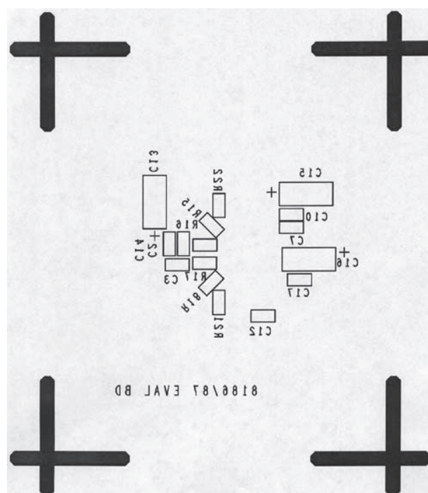
Figure 15. Circuit Side Silkscreen
