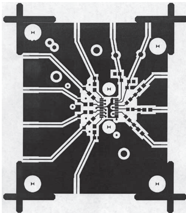
Figure 12. Component Side Board Layout
