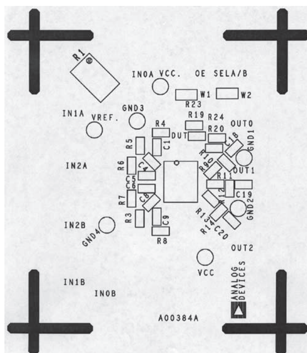
Figure 14. Component Side Silkscreen
