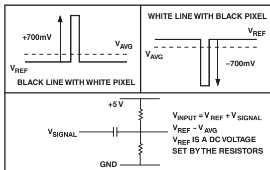
Figure 7. Pathological Case for Input Dynamic Range
