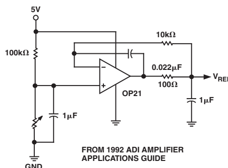
Figure 6a. Synthesis of a False Ground Reference
