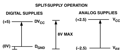
Figure 9. Split-Supply Operation
