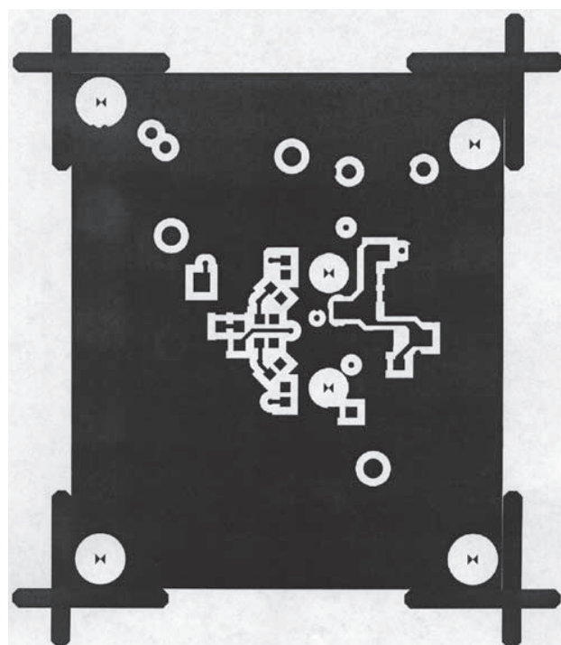
Figure 13. Circuit Side Board Layout
