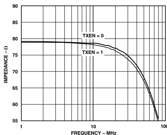
TPC 6. Output Impedance vs. Frequency
