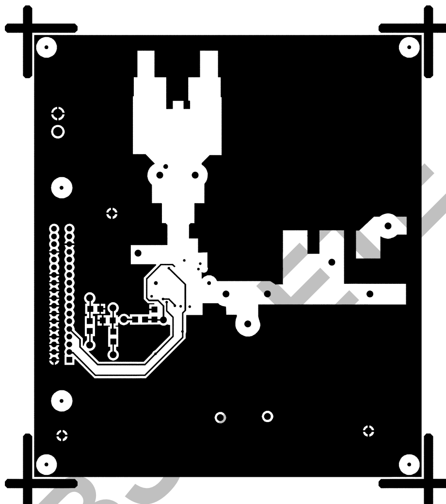
Figure 15. Evaluation Board Layout—Circuit Side
