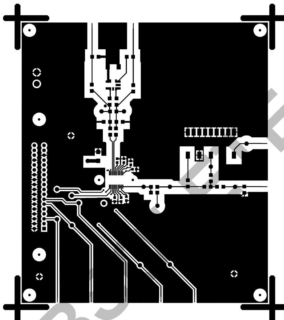
Figure 12. Evaluation Board Layout—Component Side
