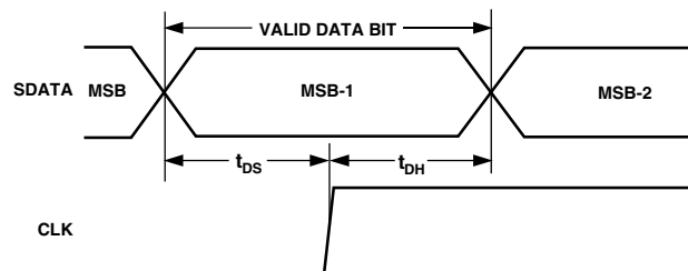
Figure 3. SDATA Timing
