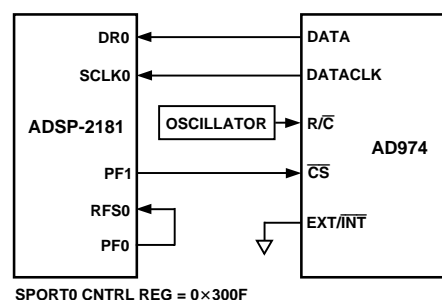
Figure 26. AD974-to-ADSP-2181 Interface
