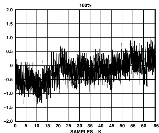
Figure 17. INL Plot
