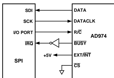
Figure 25. AD974-to-SPI Interface
