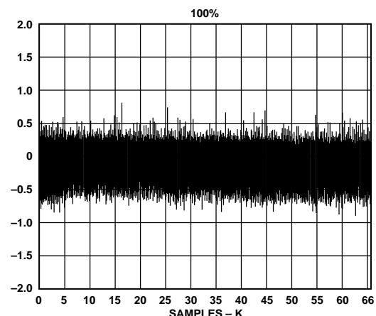
Figure 18. DNL Plot
