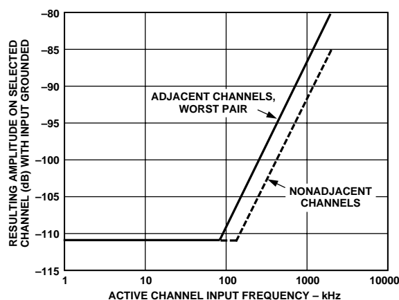
Figure 22. Crosstalk vs. Input Frequency (kHz)
