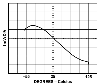
Figure 13. Reference Drift
