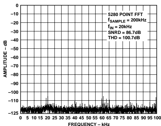
Figure 16. FFT Plot
