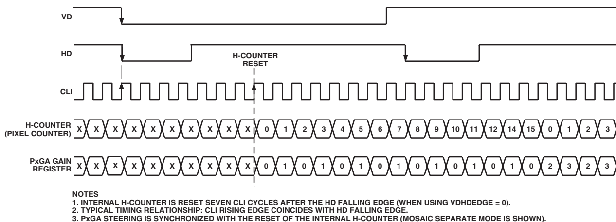
Figure 13. H-Counter Synchronization
