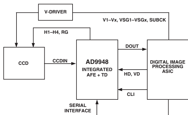
Figure 1. Typical Application
