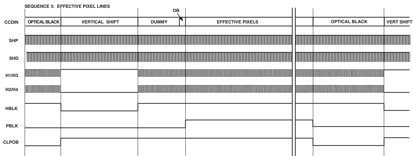
Figure 27. Horizontal Sequences during Effective Pixels
