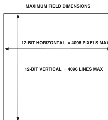
Figure 2a. Vertical and Horizontal Counters
