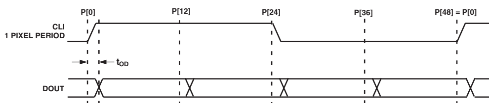
Figure 6. H-Clock Inverse Phase Relationship
