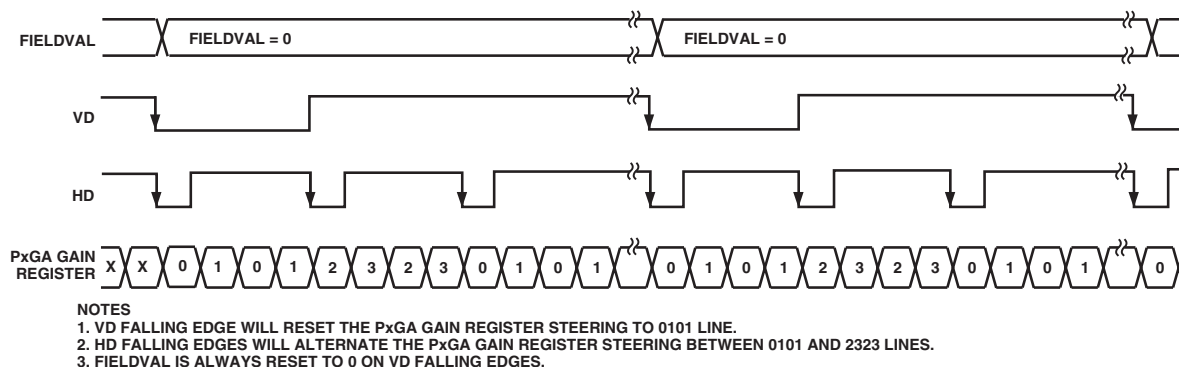
Figure 18a. PxGA Color Steering—Progressive Mode
