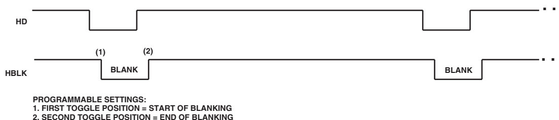
Figure 9. Horizontal Blanking (HBLK) Pulse Placement
