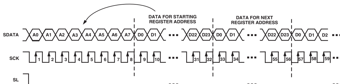
Figure 3a. Serial Write Operation
