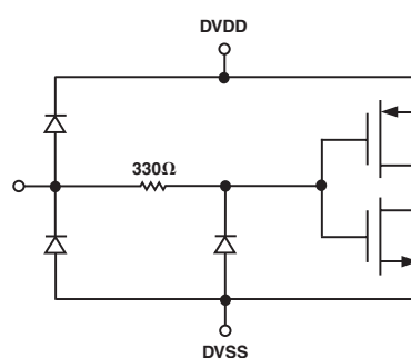
Circuit 4. Digital Inputs (Pins 31-35, 38)
