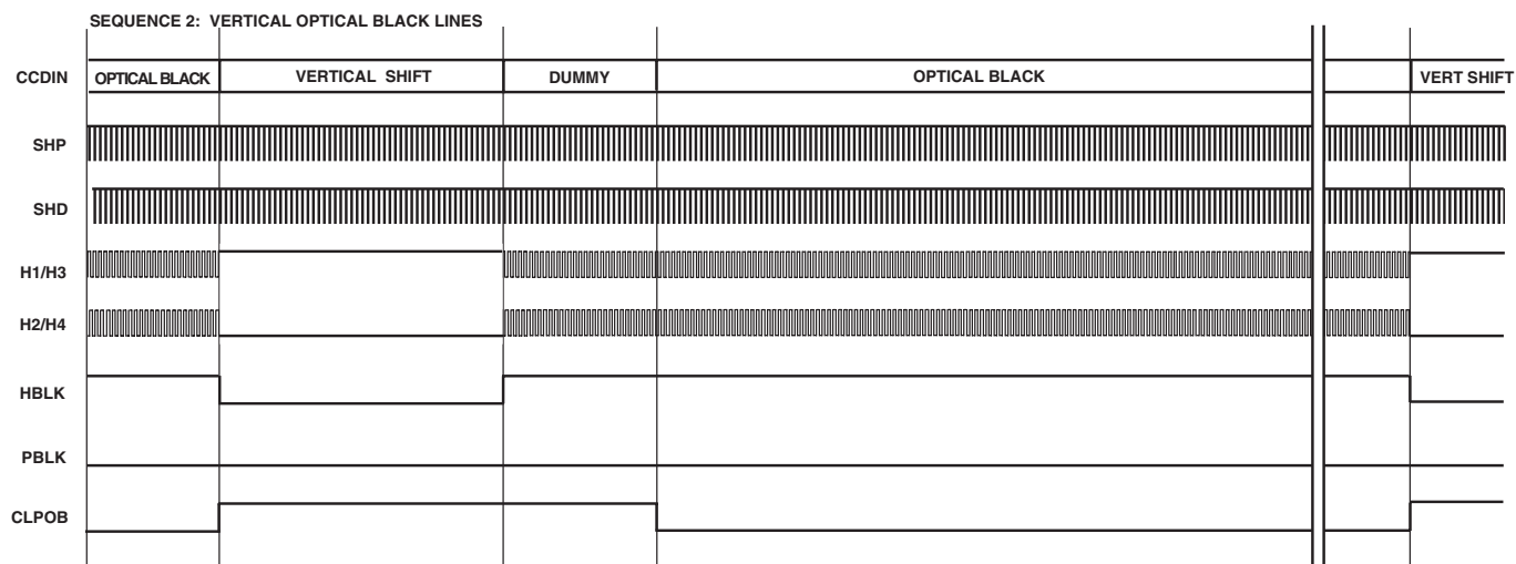
Figure 26. Horizontal Sequences during Vertical Optical Black Pixels
