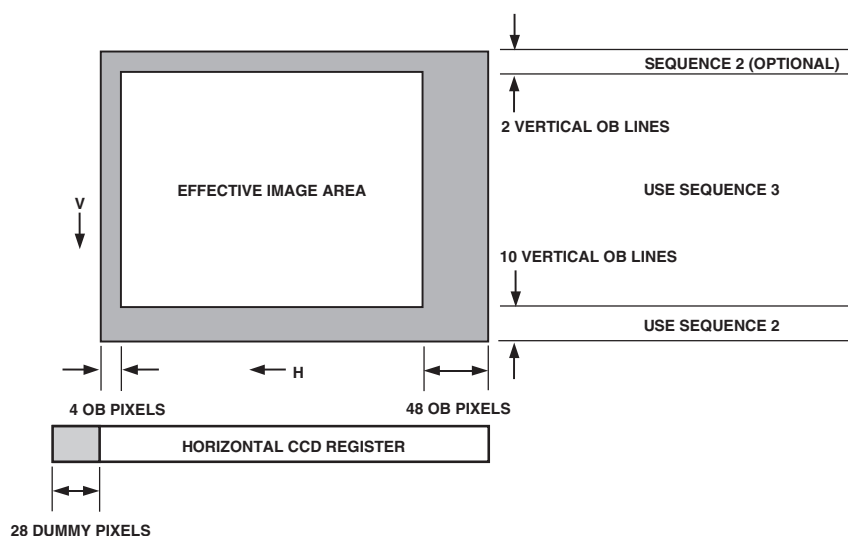
Figure 24. Example CCD Configuration
