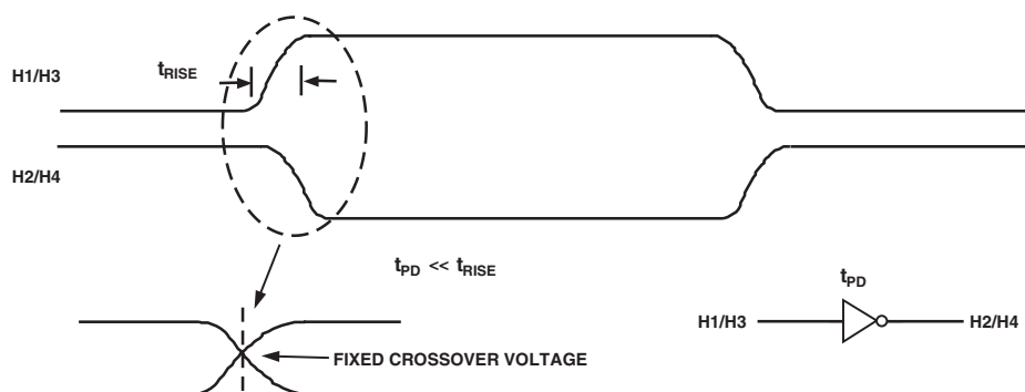
Figure 6. H-Clock Inverse Phase Relationship
