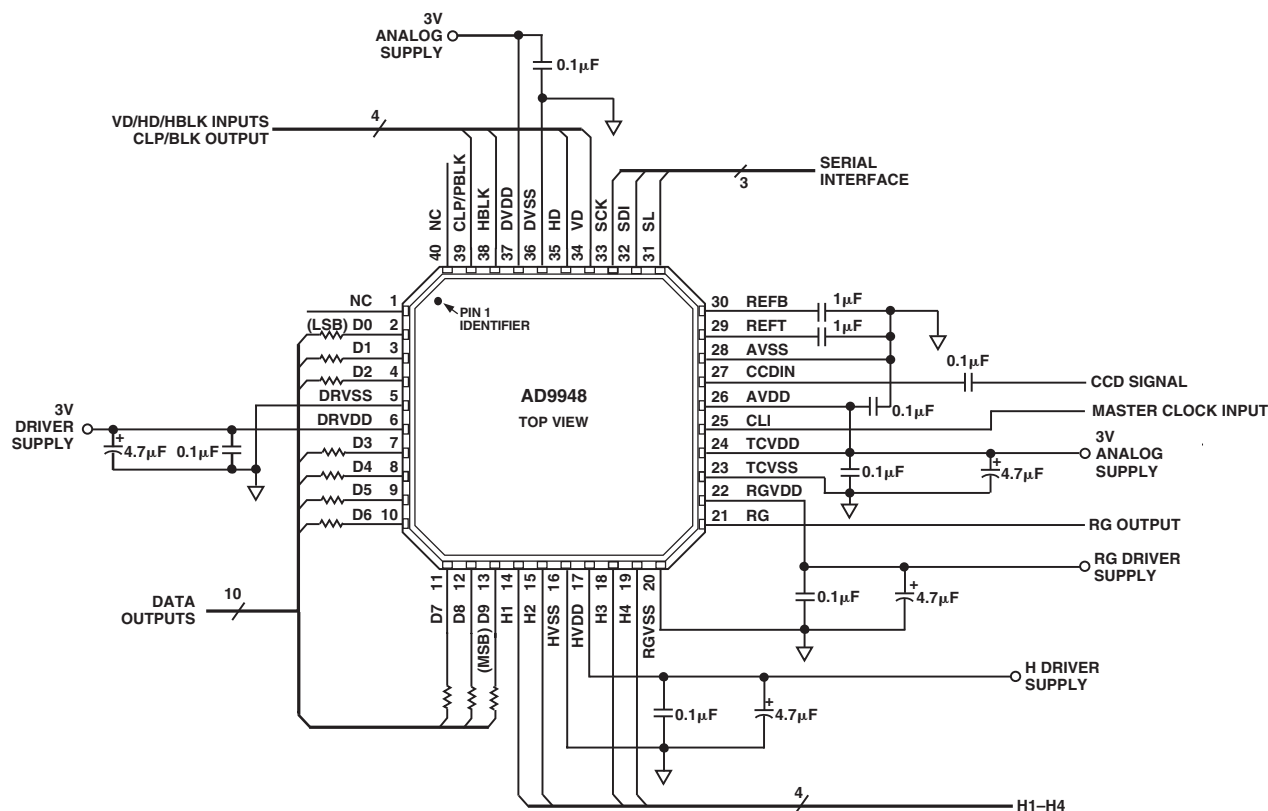
Figure 21. Recommended Circuit Configuration
