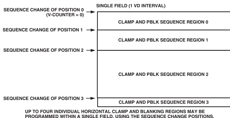
Figure 12. Clamp and Blanking Sequence Flexibility
