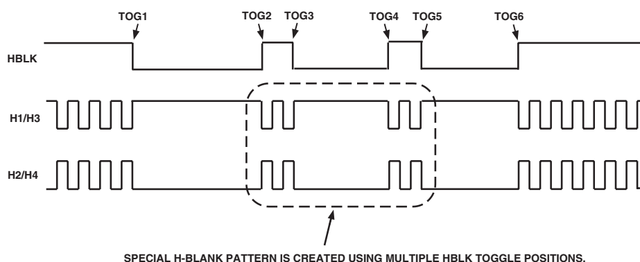
Figure 11. Generating Special HBLK Patterns
