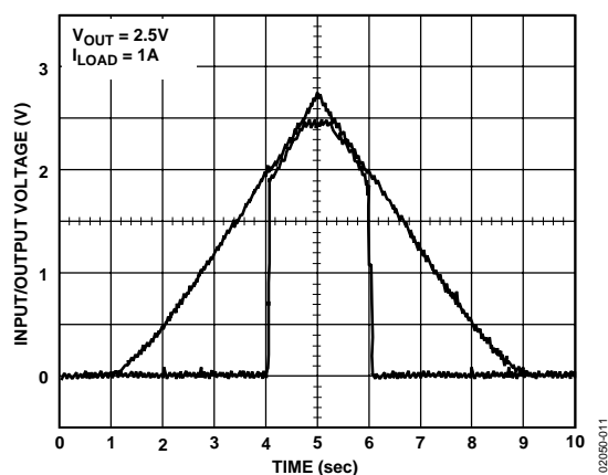
Figure 11. Power-Up/Power-Down
