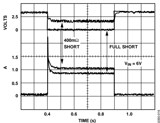
Figure 16. Short-Circuit Current
