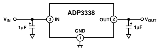
Figure 2. Typical Application Circuit
