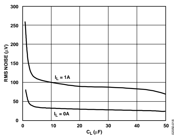
Figure 18. RMS Noise vs. C_L
