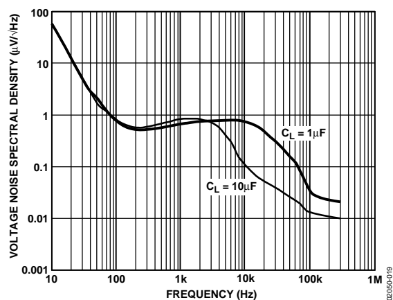
Figure 19. Output Noise Density (10 Hz to 100 kHz)
