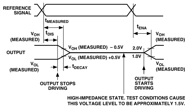
Figure 20. Output Enable/Disable
