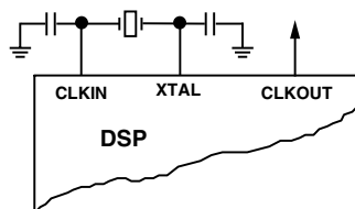
Figure 3. External Crystal Connections
