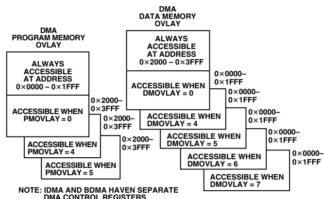
Figure 11. Direct Memory Access—PM and DM Memory Maps
