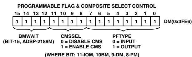
Figure 7. Programmable Flag and Composite Select Control Register
