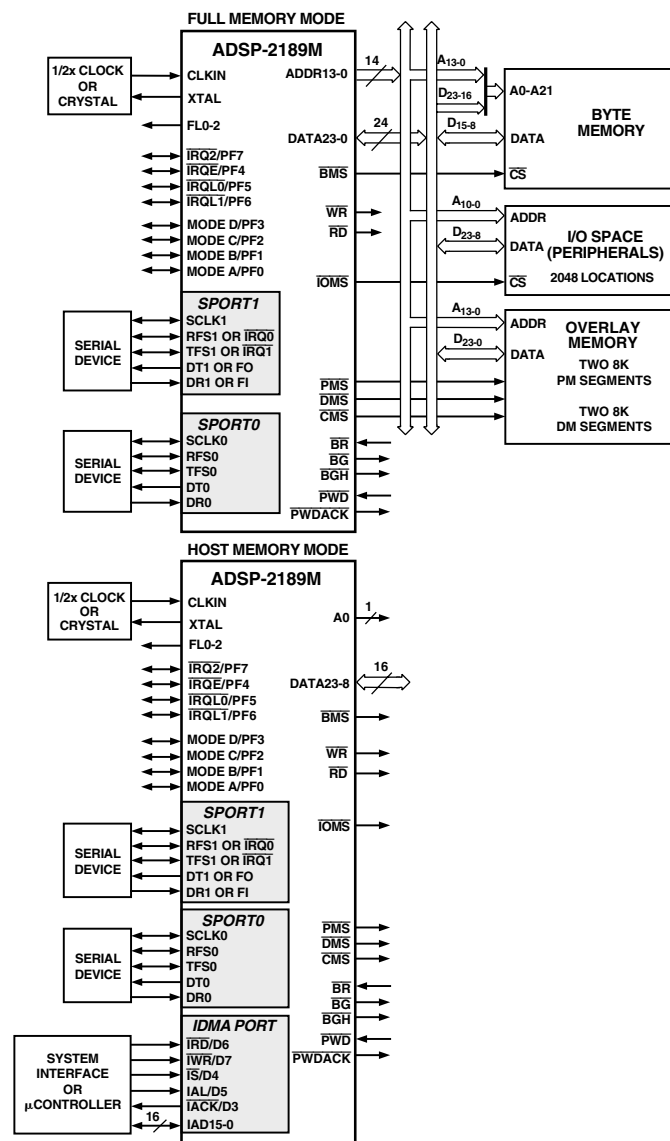
Figure 2. ADSP-2189M Basic System Interface
