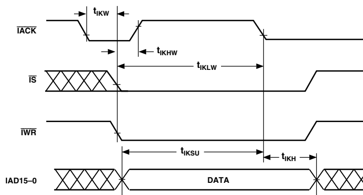
Figure 30. IDMA Write, Long Write Cycle
