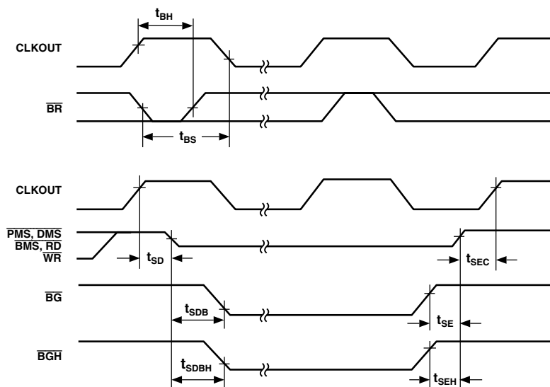
Figure 24. Bus Request–Bus Grant
