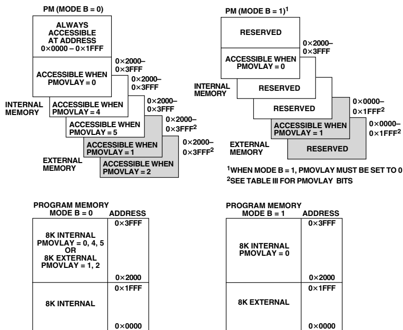
Figure 4. Program Memory
