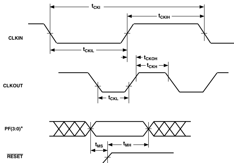
Figure 22. Clock Signals
