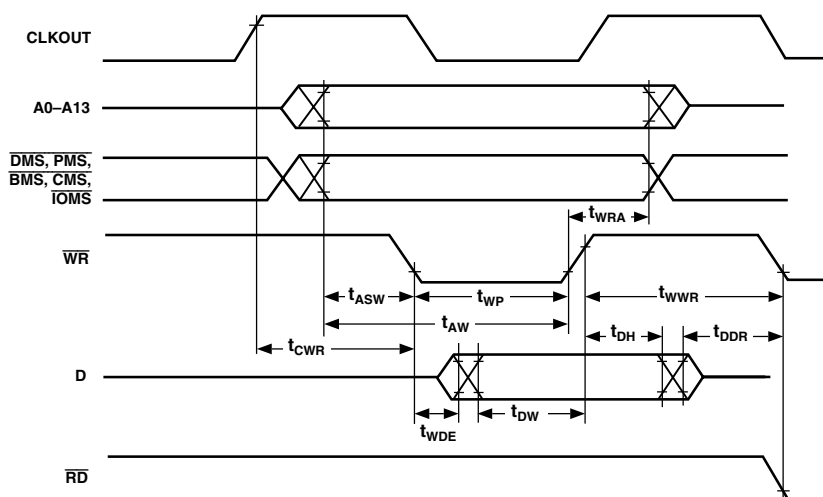
Figure 26. Memory Write
