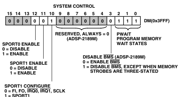
Figure 8. System Control Register
