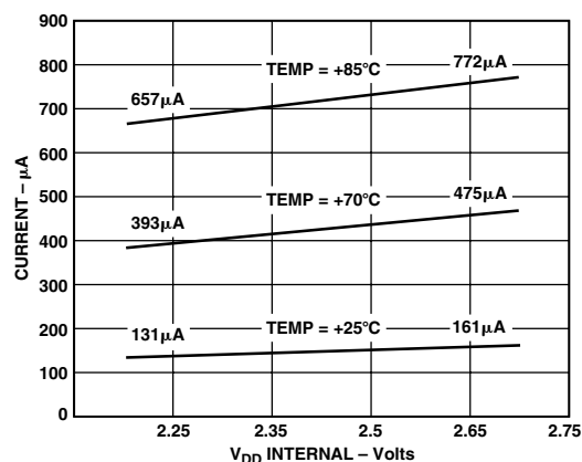
Figure 18. I_{DD} Power-Down
