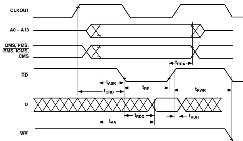
Figure 25. Memory Read
