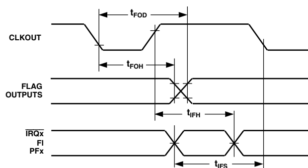
Figure 23. Interrupts and Flags
