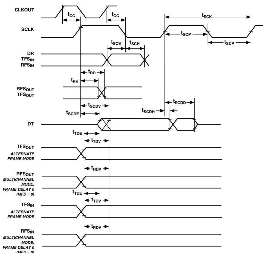
Figure 27. Serial Ports
