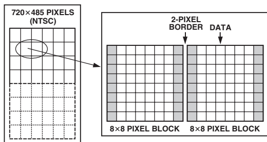
Figure 50. DNR Border Area
