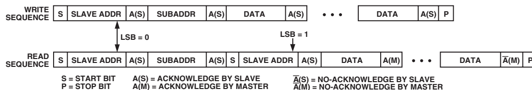
Figure 20. Read and Write Sequence
