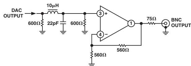
Figure 55. Example of Output Filter for SD, 16x Oversampling
