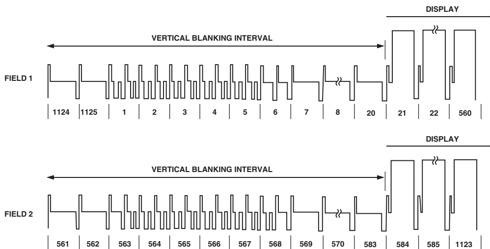
Figure 117. SMPTE 274M (1080i)
