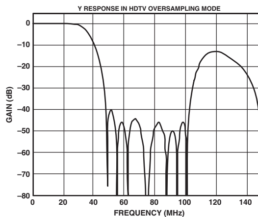
TPC 6. HDTV—Y (2× Oversampling Filter)
