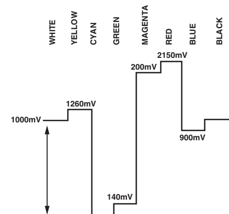
Figure 103. U Levels—PAL
