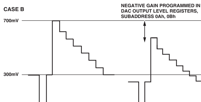
Figure 40. Programmable DAC Gain—Positive and Negative Gain
