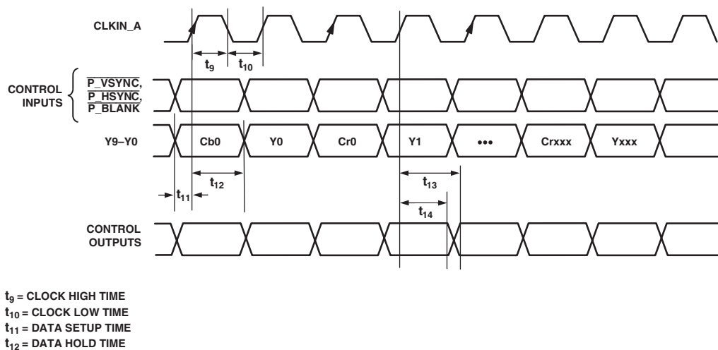
Figure 5. PS 4:2:2 1 × 10-Bit Interleaved at 54 MHz \overline{\text{HSYNC}}/\overline{\text{VSYNC}} Input Mode [Input Mode 111]
