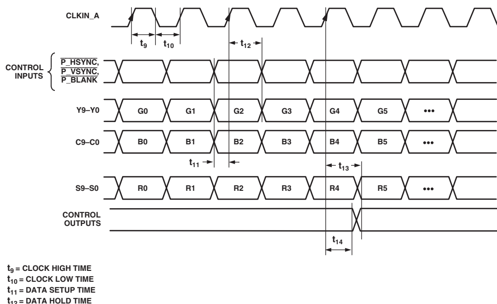
Figure 3. HD RGB 4:4:4 Input Mode [Input Mode 010]
