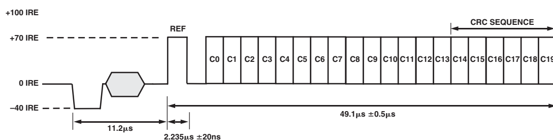
Figure 63. Standard Definition CGMS Waveform Diagram
