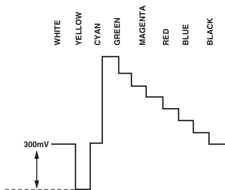
Figure 105. Y Levels—PAL
