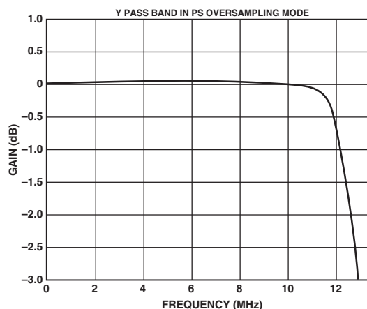
TPC 4. PS—Y 8× Oversampling Filter (Pass Band)
