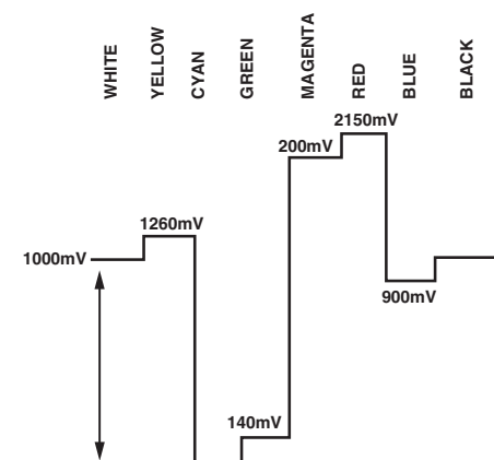
Figure 102. U Levels—NTSC
