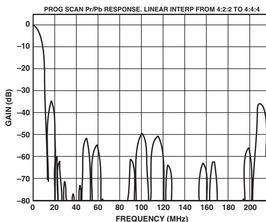
TPC 1. PS—UV 8× Oversampling Filter (Linear)
