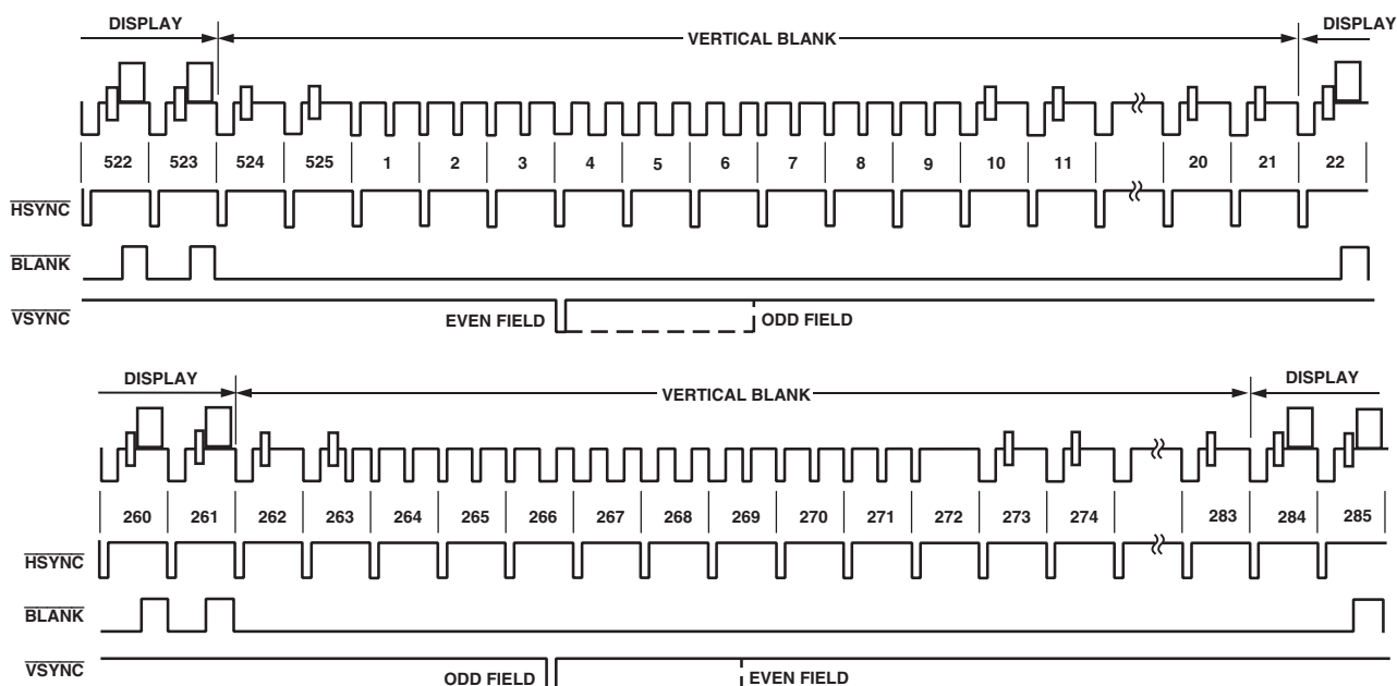
Figure 85. SD Slave Mode 2 (NTSC)
