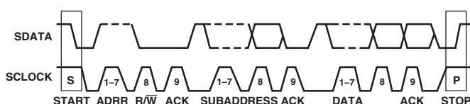
Figure 19. Bus Data Transfer
