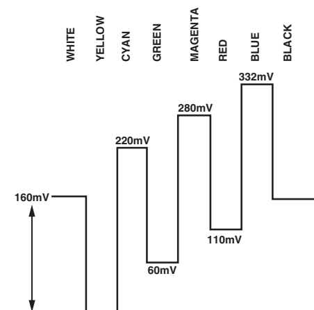
Figure 101. U Levels—PAL
