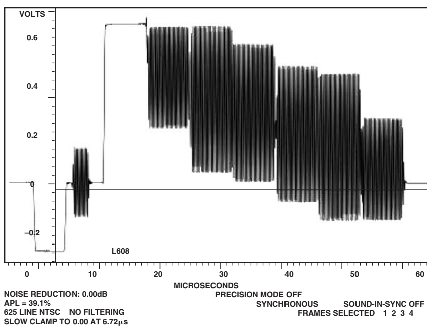
Figure 109. PAL Color Bars 75%
