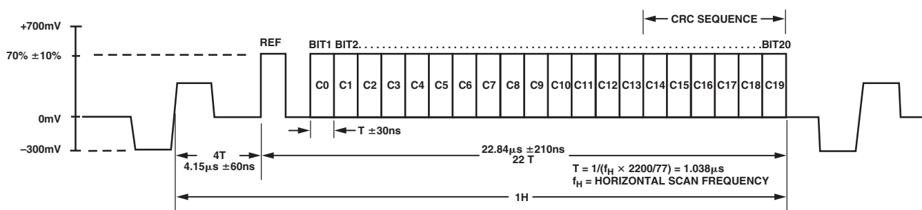
Figure 65. HDTV 1080i CGMS Waveform
