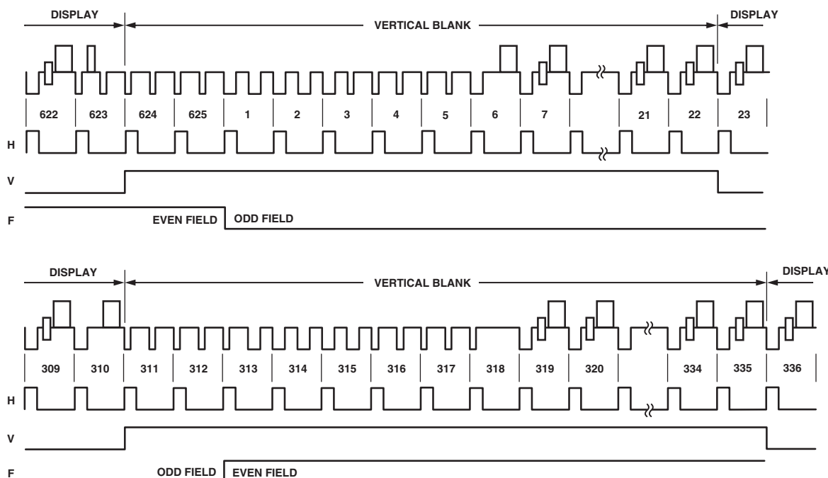
Figure 80. SD Master Mode 0, PAL
