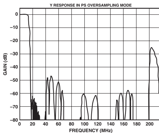
TPC 3. PS—Y (8× Oversampling Filter)
