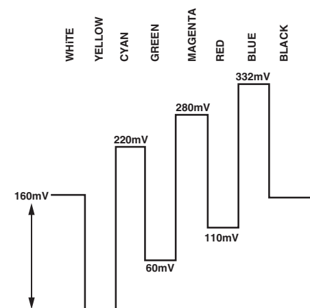
Figure 100. U Levels—NTSC
