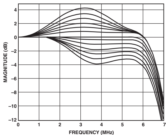
TPC 13. Luma SSAF Filter—Programmable Responses
