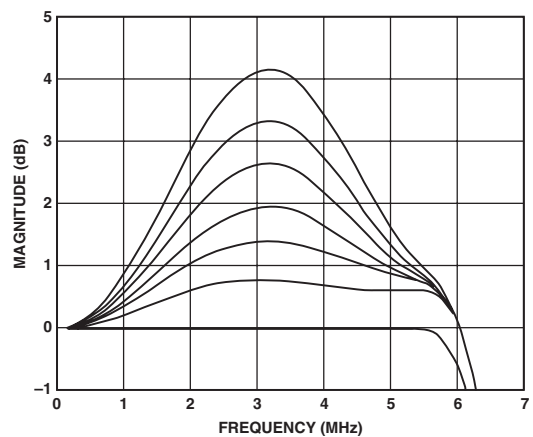
TPC 14. Luma SSAF Filter—Programmable Gain
