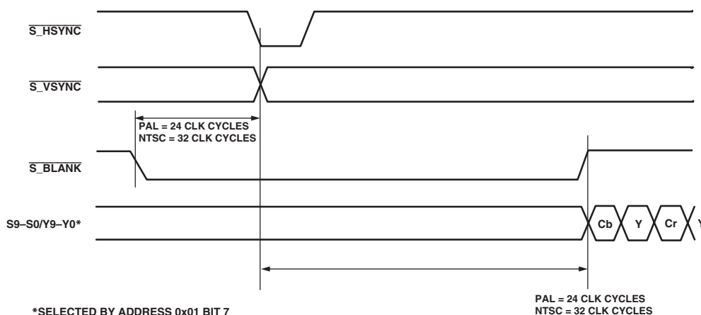
Figure 15. SD Timing Input for Timing Mode 1
