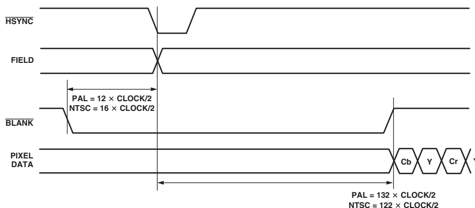
Figure 84. SD Timing Mode 1—Odd/Even Field Transitions Master/Slave
