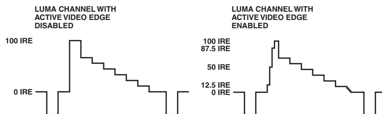
Figure 52. Example of Active Video Edge Functionality
