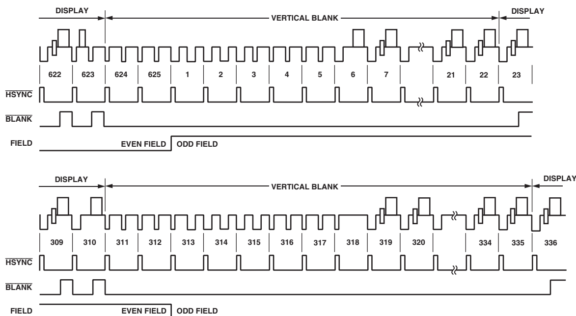
Figure 90. SD Timing Mode 3 (PAL)
