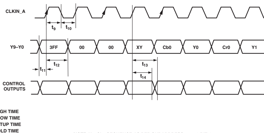
Figure 7. PS Only 4:2:2 1 × 10-Bit Interleaved at 54 MHz EAV/SAV Input Mode [Input Mode 111]
