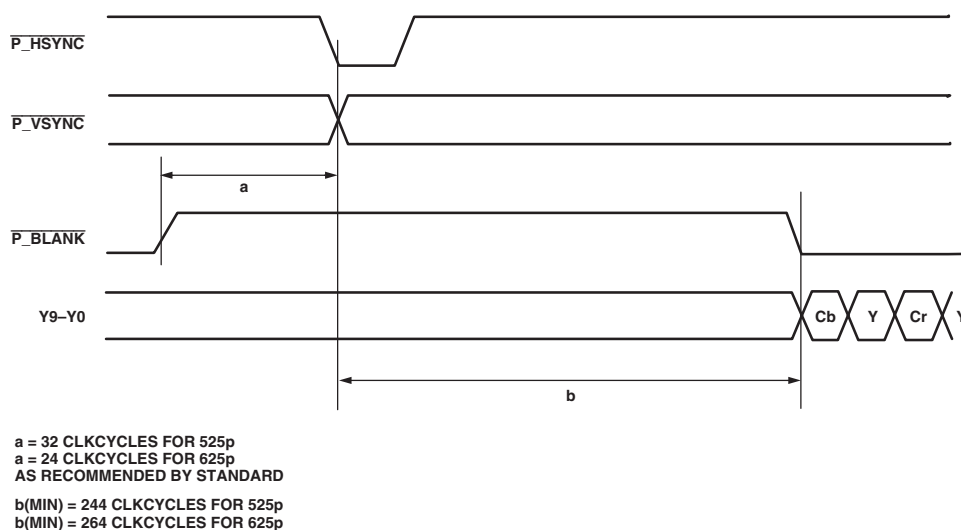
Figure 14. PS 4:2:2 1 \times 10 -Bit Interleaved Input Timing Diagram
