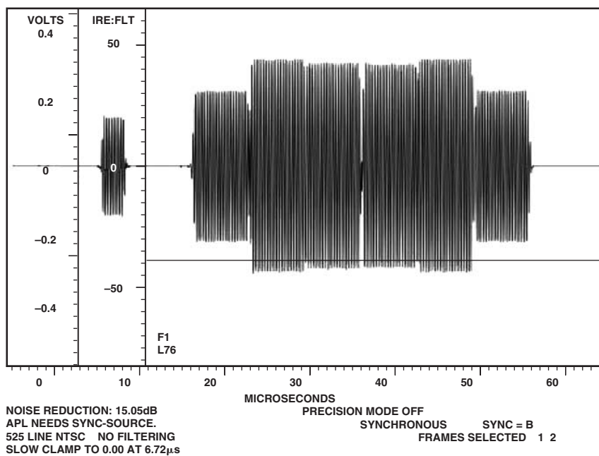
Figure 107. NTSC Chroma
