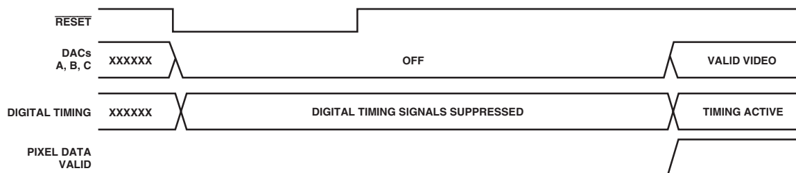
Figure 33. \overline{\text{RESET}} Timing Sequence
