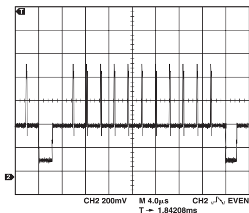
Figure 73. 625p Hatch Pattern
