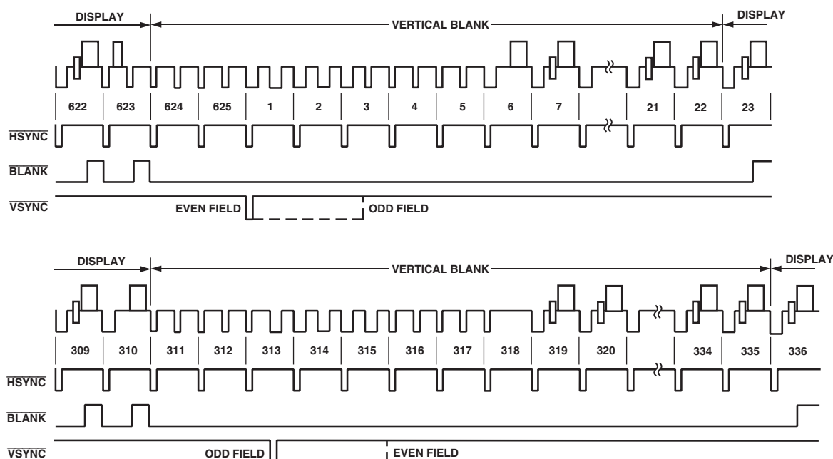
Figure 86. SD Slave Mode 2 (PAL)
