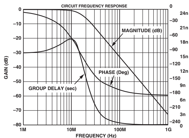
Figure 56. Filter Plot for Output Filter for SD, 16x Oversampling
