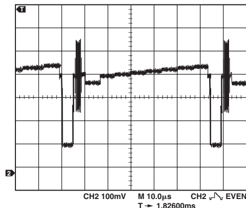
Figure 71. PAL Black Bar [−21 mV, 0 mV, 3.5 mV, 7 mV, 10.5 mV, 14 mV, 18 mV, 23 mV]
