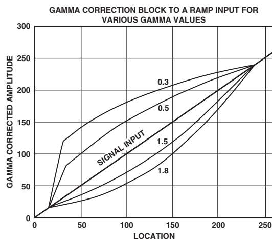
Figure 42. Signal Input (Ramp) and Selectable Output Curves
