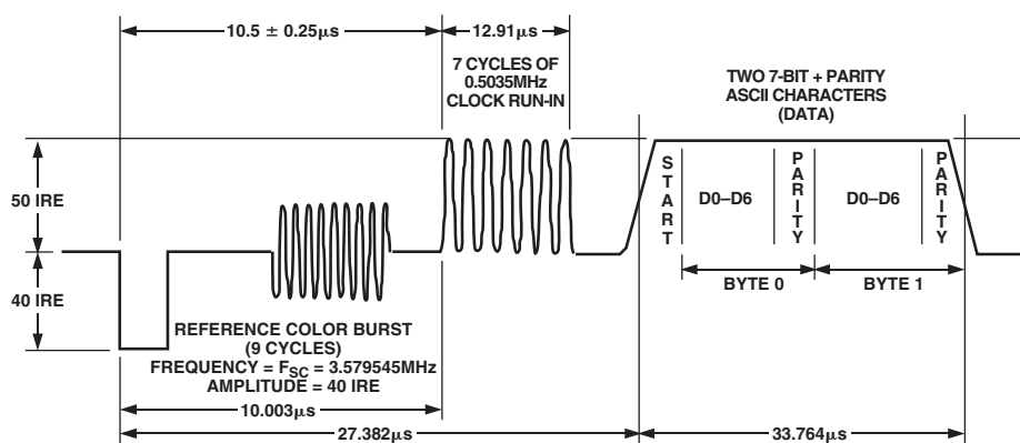
Figure 67. Closed Captioning Waveform, NTSC
