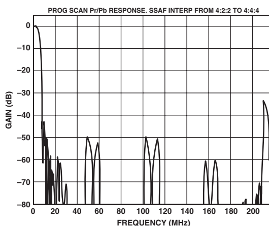
TPC 2. PS—UV 8× Oversampling Filter (SSAF)
