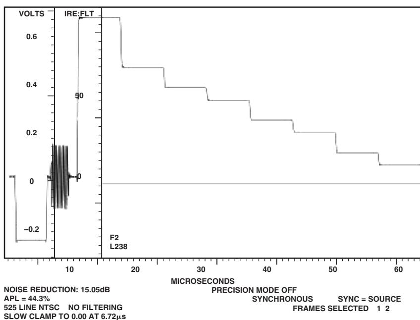
Figure 108. NTSC Luma
