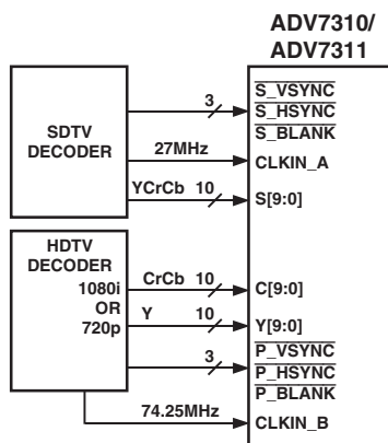
Figure 25. Simultaneous HD and SD Input
