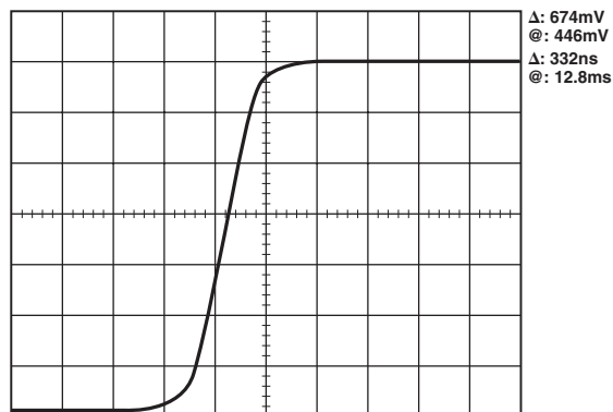
Figure 47. Output Signal from Adaptive Filter Control
