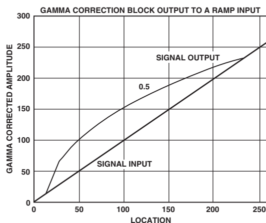
Figure 41. Signal Input (Ramp) and Signal Output for Gamma 0.5
