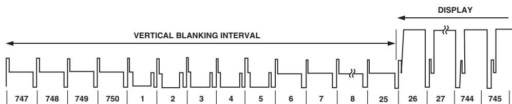
Figure 116. SMPTE 296M (720p)
