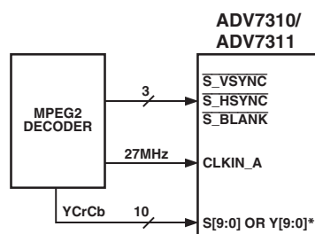
Figure 22. SD Only Input Mode
