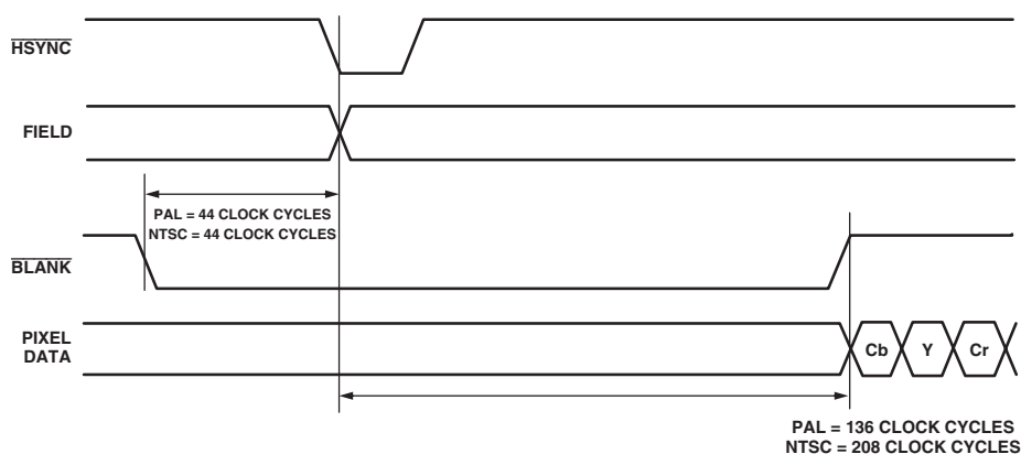
Figure 35. Active Pixel Timing
