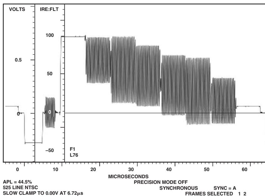
Figure 106. NTSC Color Bars 75%
