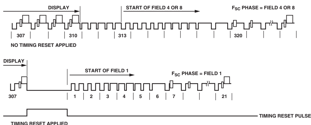
Figure 30. Timing Reset Timing Diagram
