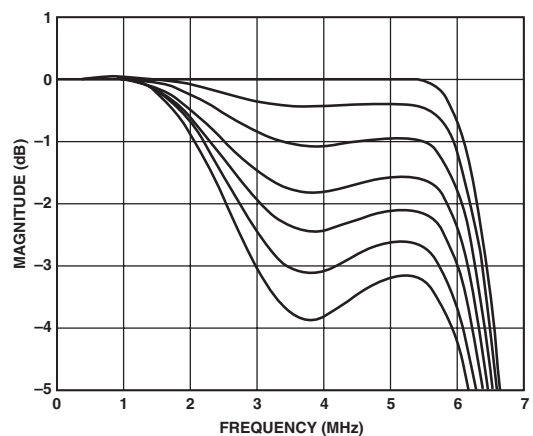
TPC 15. Luma SSAF Filter—Programmable Attenuation
