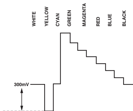
Figure 104. Y Levels—NTSC
