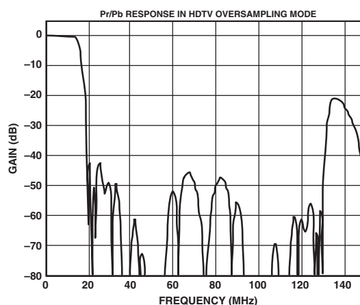
TPC 5. HDTV—UV (2× Oversampling Filter)
