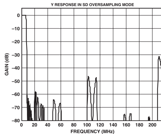
TPC 11. Y-16x Oversampling Filter
