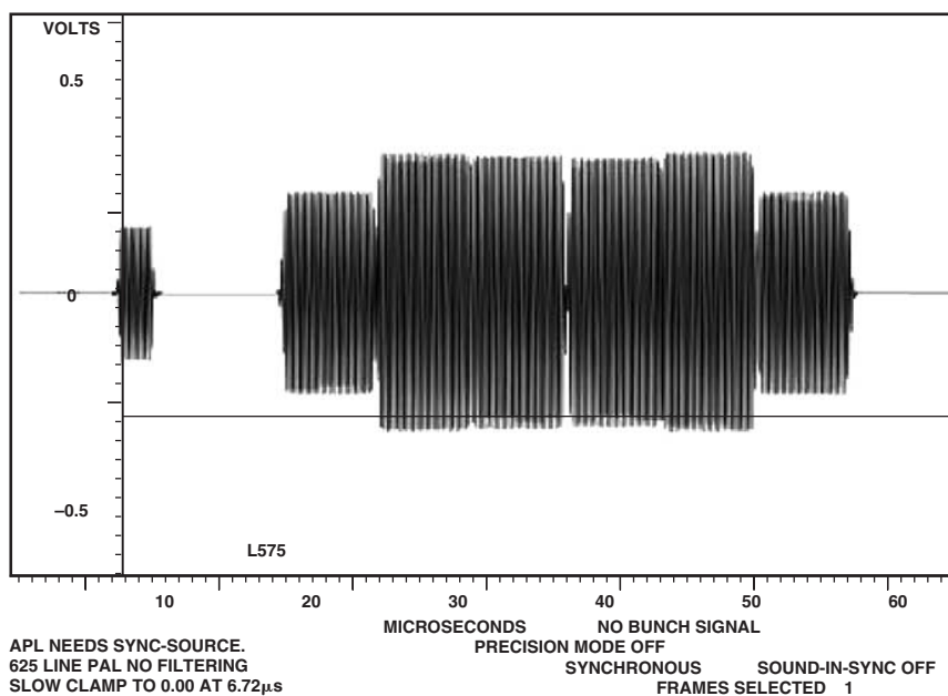
Figure 110. PAL Chroma
