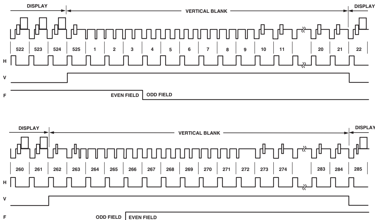
Figure 79. SD Master Mode 0, NTSC
