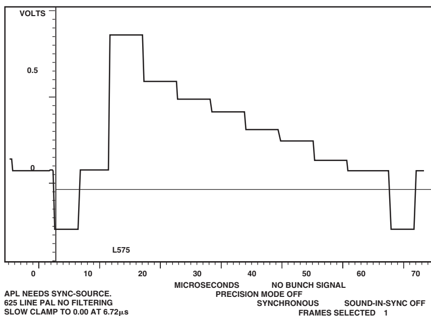
Figure 111. PAL Luma
