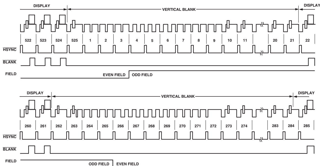
Figure 89. SD Timing Mode 3 (NTSC)
