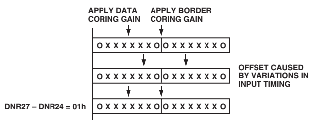
Figure 49. DNR Offset Control
