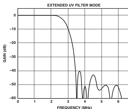
Figure 38. UV SSAF Filter
