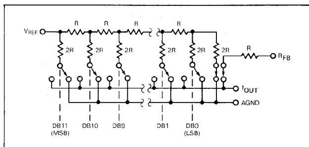
FIGURE 1: Simplified D/A Circuit
