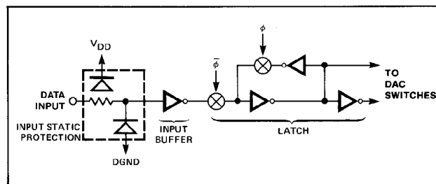
FIGURE 3: Digital Input Structure For One Bit
