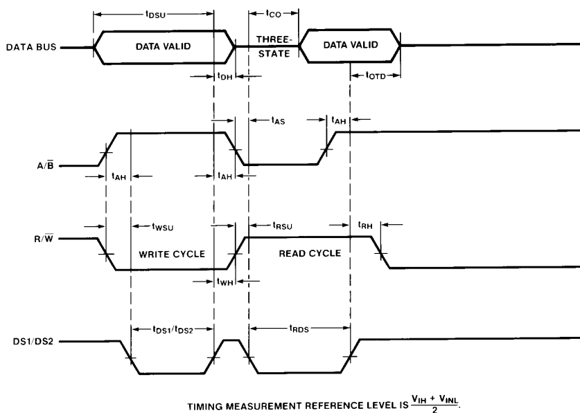
Timing Diagram
