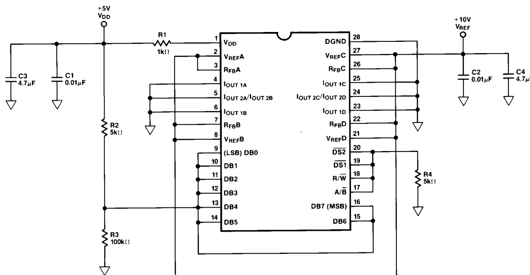
Burn-in Circuit
