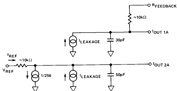
Figure 4. Equivalent DAC Circuit (All Digital Inputs LOW)
