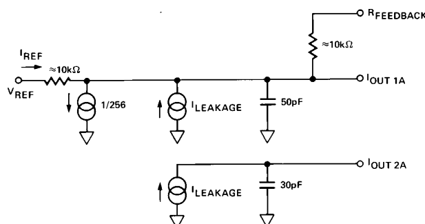
Figure 3. Equivalent DAC Circuit (All Digital Inputs HIGH)
