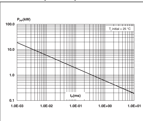
Figure 4. Peak pulse power versus exponential pulse duration
