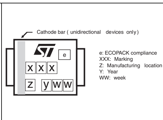
Figure 14. Marking layout (1)
