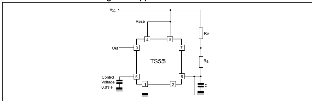
Figure 6. Application schematic
