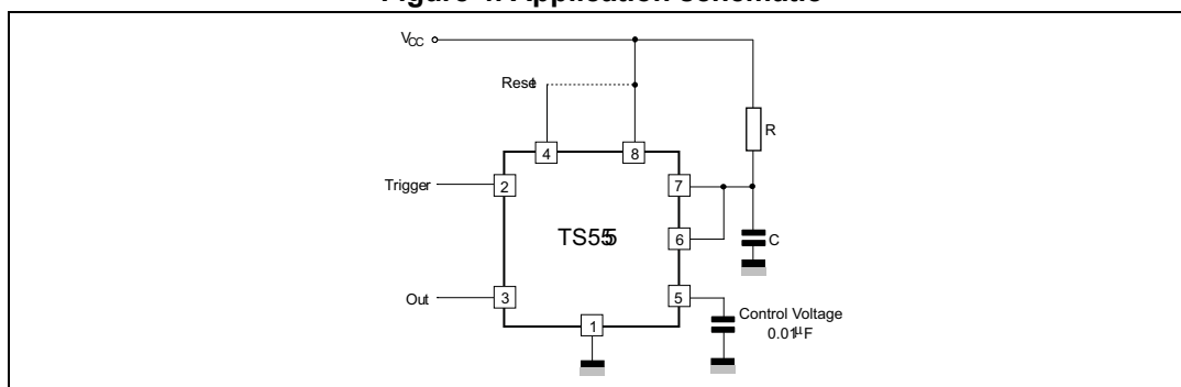
Figure 4. Application schematic
