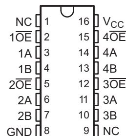
DBQ Package 16-Pin SSOP Top View
