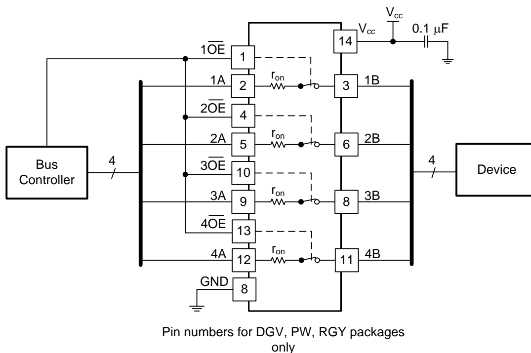
Figure 5. Typical Application of the SN74CB3Q3125
