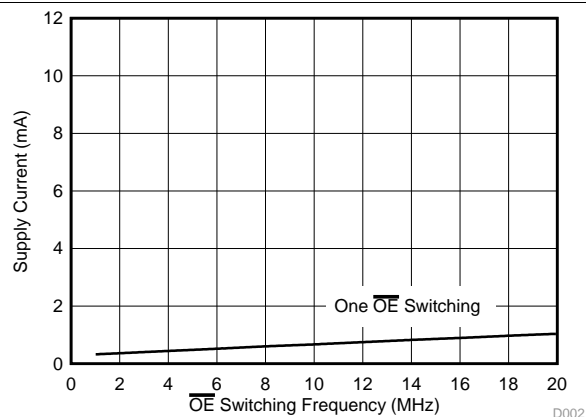
Figure 2. Typical Supply Current vs \overline{\text{OE}} Switching Frequency
