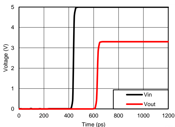
Figure 6. Propagation Delay ( t_{pd} ) Simulation Result at V_{CC} = 3.3 V
