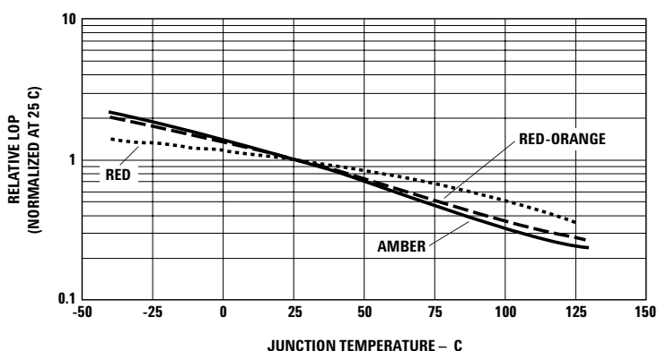
Figure 8. Relative light output vs. junction temperature
