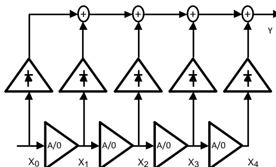
Figure 72. Logarithmic Amplifier
