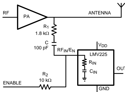
Figure 66. Typical LMV225 Application with High Resistive Tap
