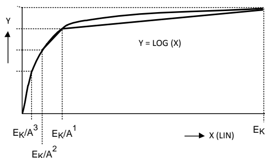
Figure 74. Log-Function on Lin Scale
