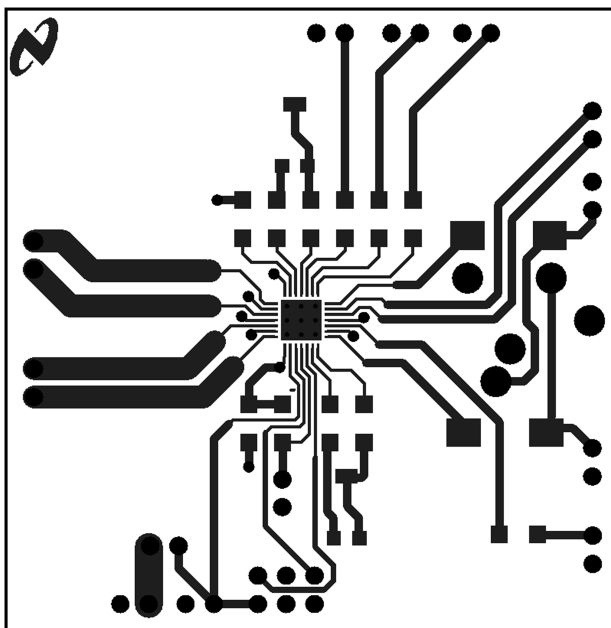
Figure 62. Recommended UQFN PCB Layout: Top Layer
