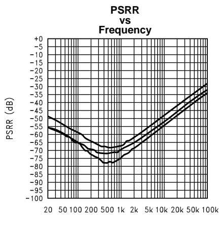
Figure 24. V_{DD} = 5V ; LLS, RLS; R_L = 8\Omega ; 0dB Gain; All audio inputs terminated; Top-Mode 12, 13; Mid-Mode 2, 3; Bot-Mode 7, 8
