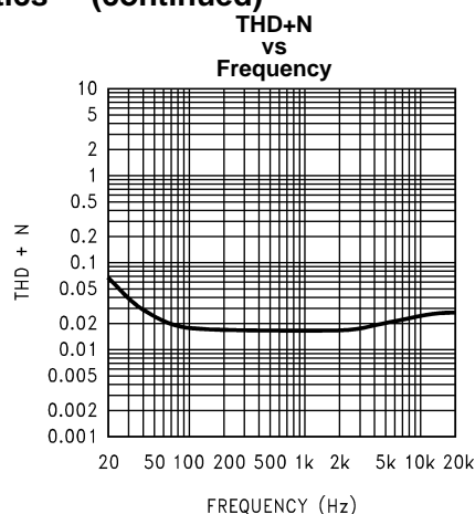
Figure 17. V_{DD} = 3V ; LINEOUT; V_O = 1V_{RMS} ; R_L = 5k\Omega ; Mode 10; 0dB Gain
