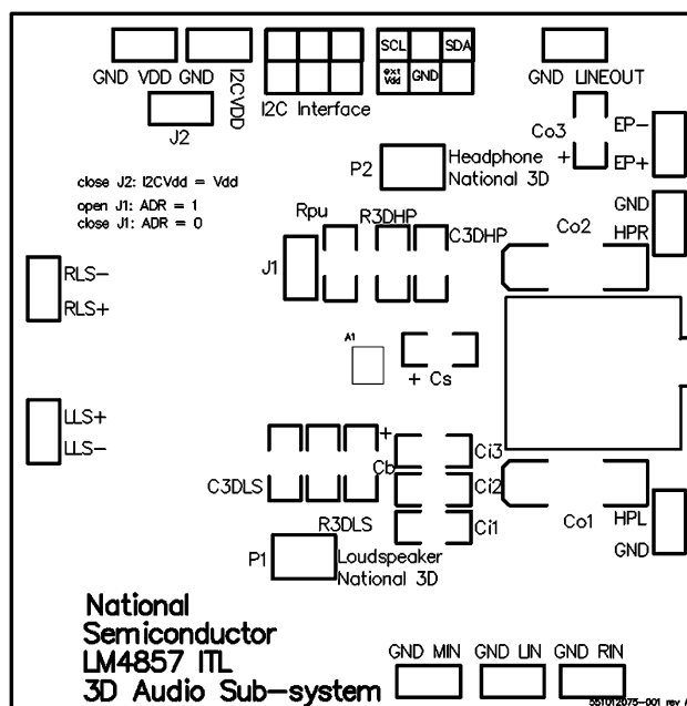
Figure 56. Recommended DSBGA PCB Layout: Top Silkscreen
