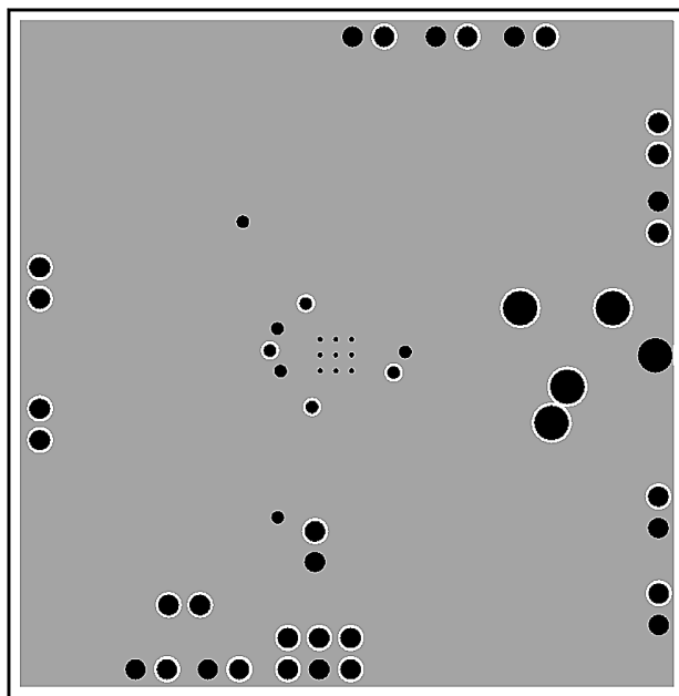
Figure 64. Recommended UQFN PCB Layout: Bottom Layer
