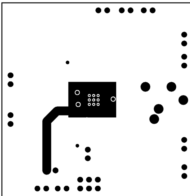
Figure 63. Recommended UQFN PCB Layout: Mid Layer
