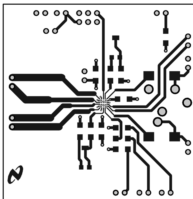
Figure 57. Recommended DSBGA PCB Layout: Top Layer
