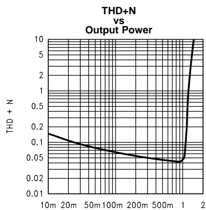
Figure 18. V_{DD} = 5V ; LLS, RLS; f = 1kHz ; R_L = 8\Omega ; Mode 7; 0dB Gain
