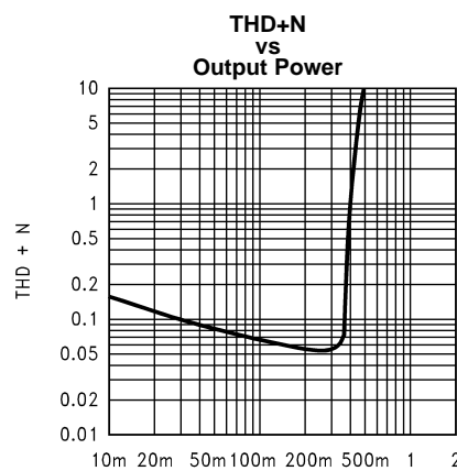
Figure 19. V_{DD} = 3V ; LLS, RLS; f = 1kHz ; R_L = 8\Omega ; Mode 7; 0dB Gain
