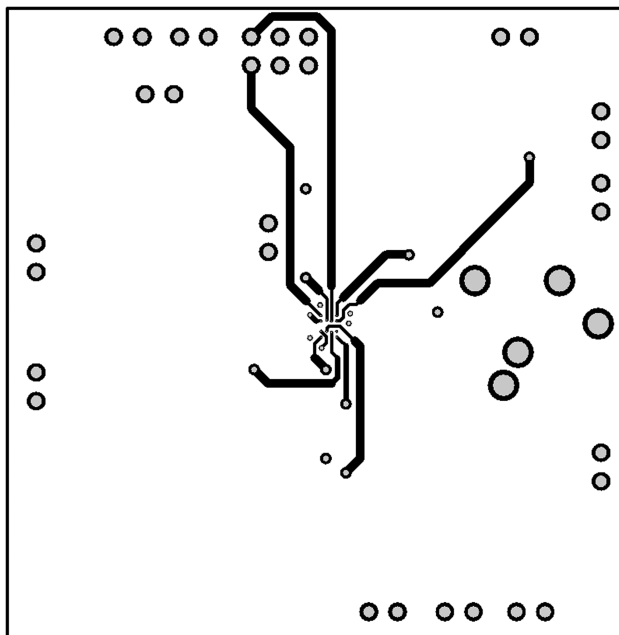
Figure 58. Recommended DSBGA PCB Layout: Inner Layer 1
