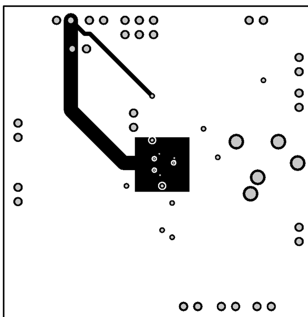
Figure 59. Recommended DSBGA PCB Layout: Inner Layer 2
