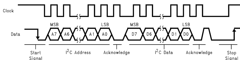
Figure 53. I²C Bus Format
